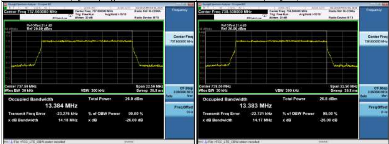
15MHz, 16QAM, Mid Channel
