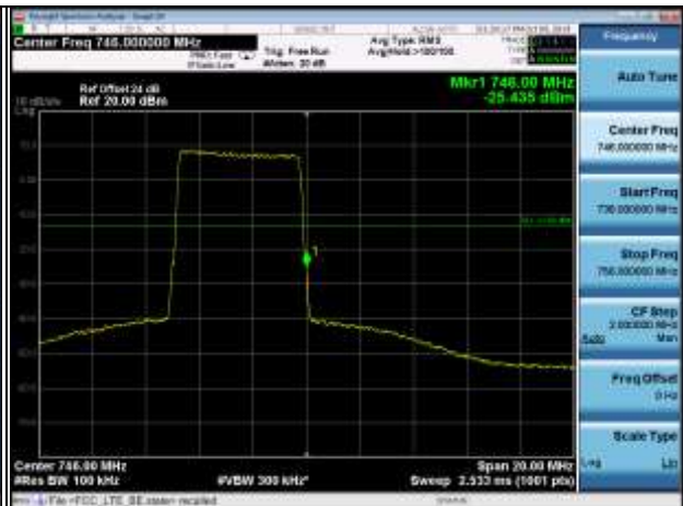
5MHz, 16QAM, High Channel
