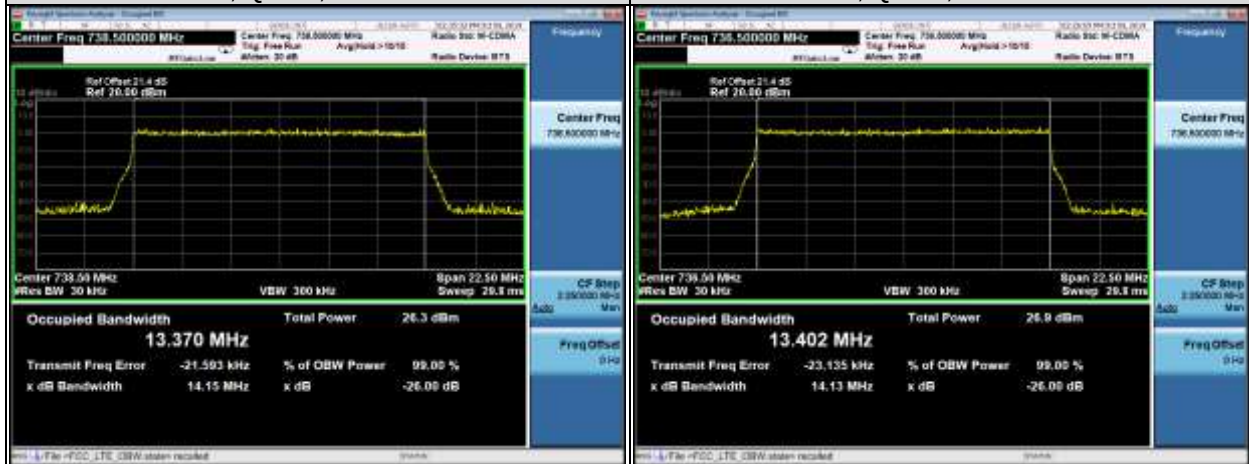
15MHz, QPSK, High Channel
