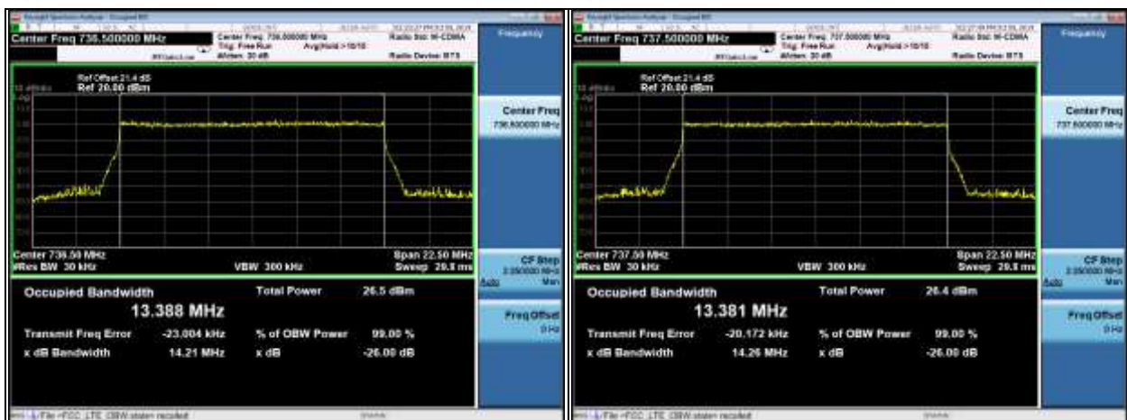
15MHz, QPSK, Low Channel
