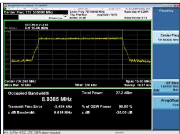
10MHz, QPSK, Mid Channel
