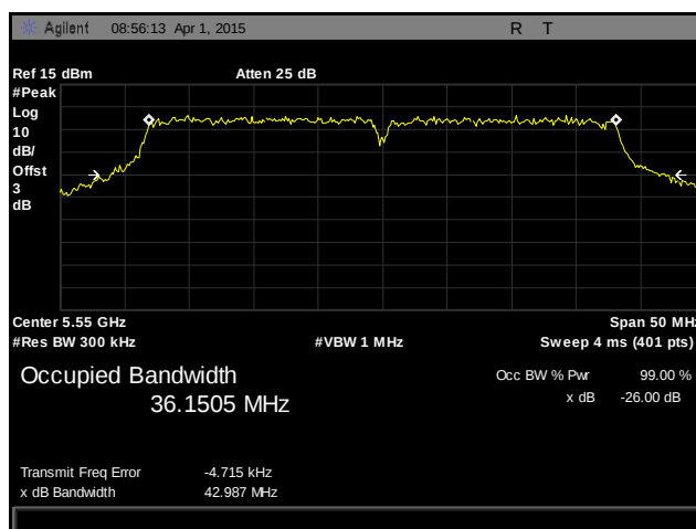
Plot 27. Occupied Bandwidth, 802.11ac 40 MHz, Mid Channel, 5550 MHz, Port A
