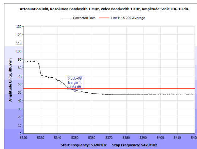
Plot 114. Radiated Band Edge, 802.11n 20 MHz, High Channel, 5320 MHz @ 5350 MHz Edge, Average
