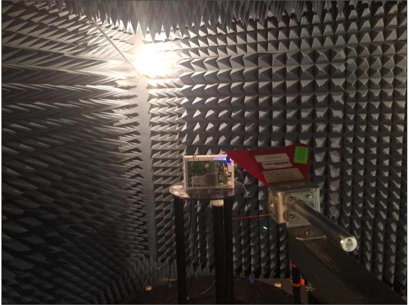
Photograph 2. Radiated Spurious Emissions, Above 1 GHz, Test Setup
