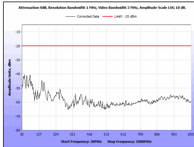
Plot 67. Radiated Spurious Emissions, Low Channel, QPSK, Port 2, 30 MHz – 1 GHz
