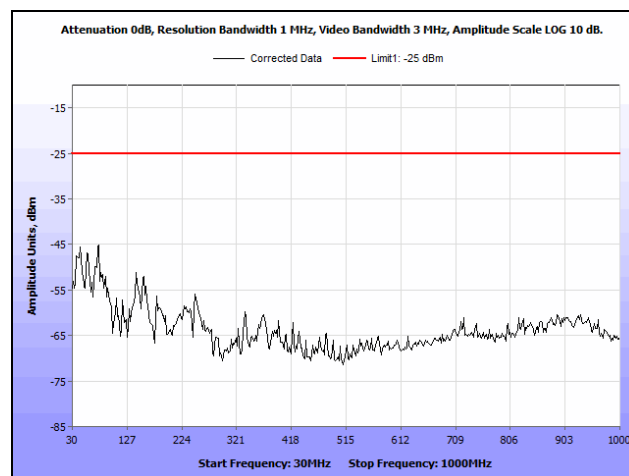
Plot 51. Radiated Spurious Emissions, Mid Channel, QPSK, Port 1, 30 MHz – 1 GHz
