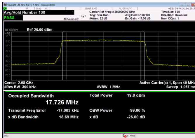
Plot 33. Occupied Bandwidth, High Channel, QAM-64, Port 2
