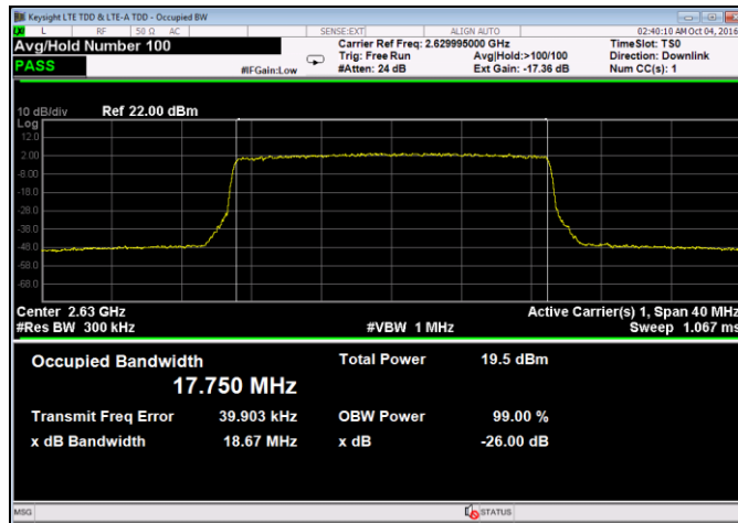
Plot 26. Occupied Bandwidth, Mid Channel, QPSK, Port 1
