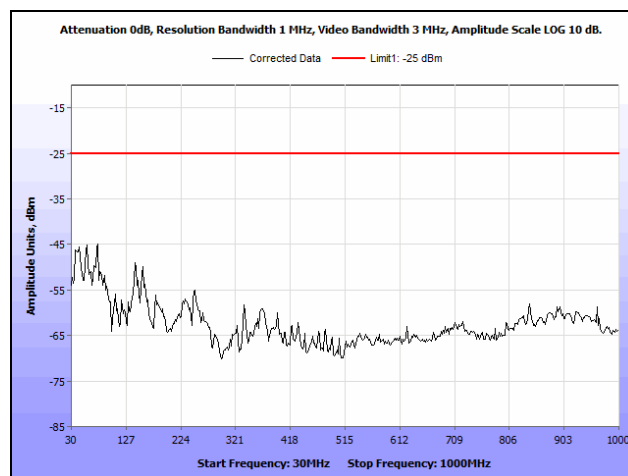
Plot 69. Radiated Spurious Emissions, Mid Channel, QPSK, Port 2, 30 MHz – 1 GHz
