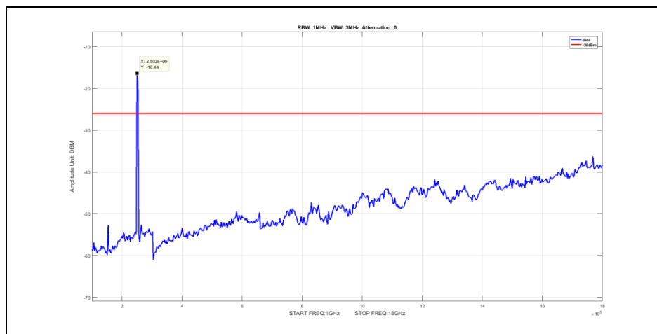
Plot 38. Radiated Spurious Emissions, Low Channel, QAM-16, Port 1, 1 GHz – 18 GHz
