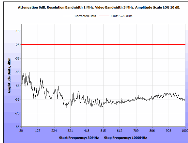
Plot 37. Radiated Spurious Emissions, Low Channel, QAM-16, Port 1, 30 MHz – 1 GHz
