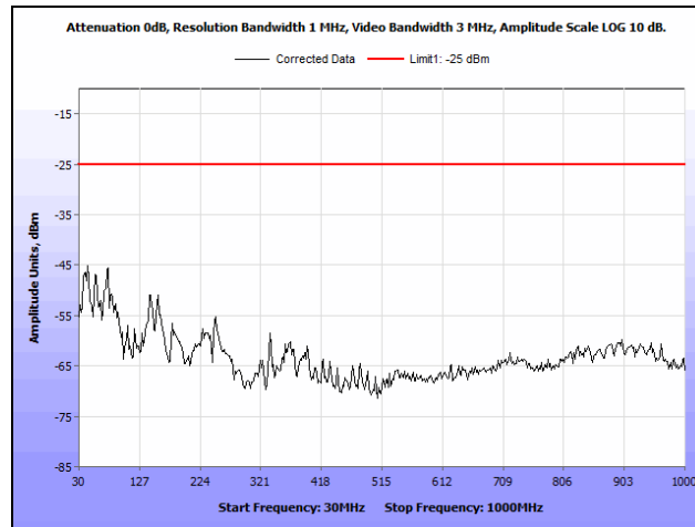
Plot 61. Radiated Spurious Emissions, Low Channel, QAM-64, Port 2, 30 MHz – 1 GHz
