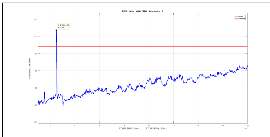
Plot 44. Radiated Spurious Emissions, Low Channel, QAM-64, Port 1, 1 GHz – 18 GHz
