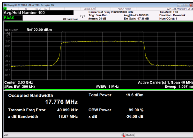
Plot 35. Occupied Bandwidth, Mid Channel, QPSK, Port 2
