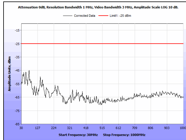
Plot 49. Radiated Spurious Emissions, Low Channel, QPSK, Port 1, 30 MHz – 1 GHz
