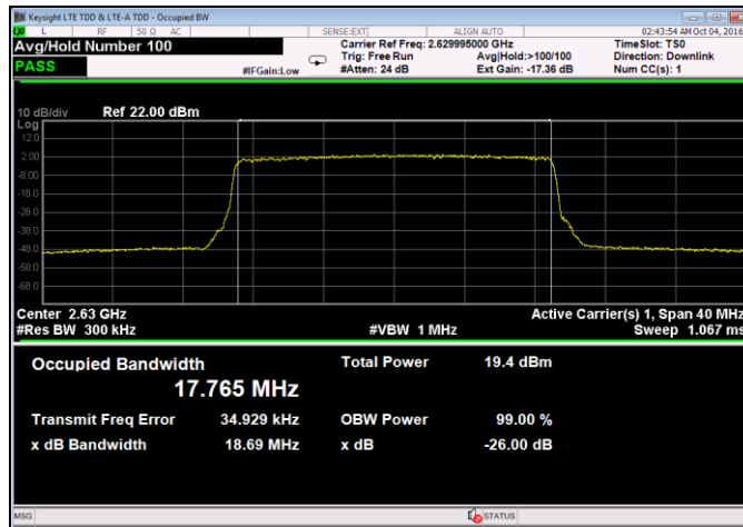
Plot 23. Occupied Bandwidth, Mid Channel, QAM-64, Port 1
