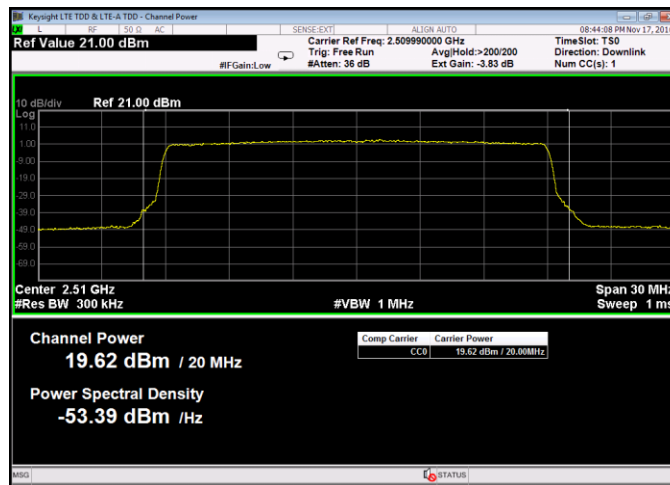
Plot 16. RF Output Power, Low Channel, QPSK, Port 2
