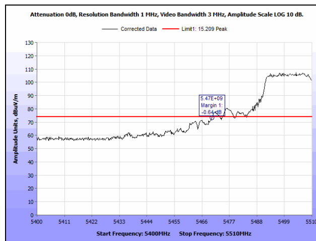
Plot 135. Radiated Band Edge, 802.11ac 40 MHz, Low Channel, 5510 MHz @ 5470 MHz Edge, Peak
