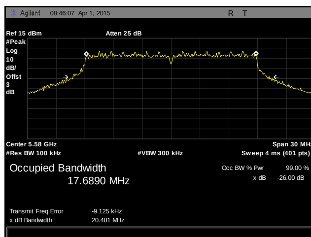
Plot 21. Occupied Bandwidth, 802.11ac 20 MHz, Mid Channel, 5580 MHz, Port A
