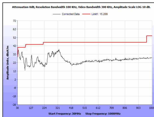
Plot 44. Radiated Spurious Emissions, 802.11n 40 MHz, Mid Channel, 2442 MHz, 30 MHz – 1 GHz
