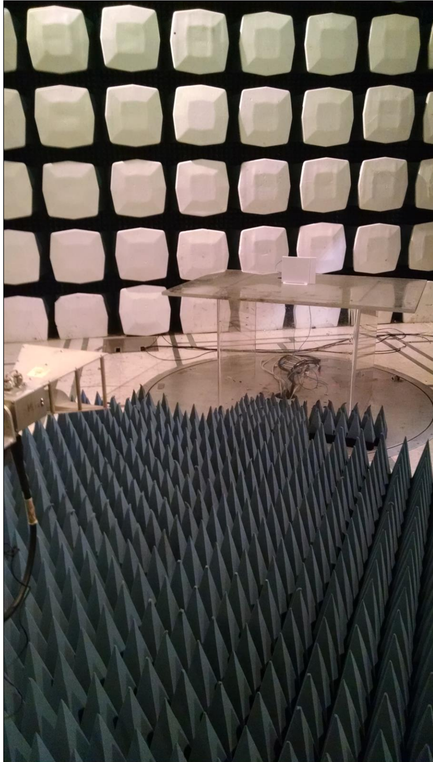
Photograph 2. Radiated Spurious Emissions, Above 1 GHz, Test Setup
