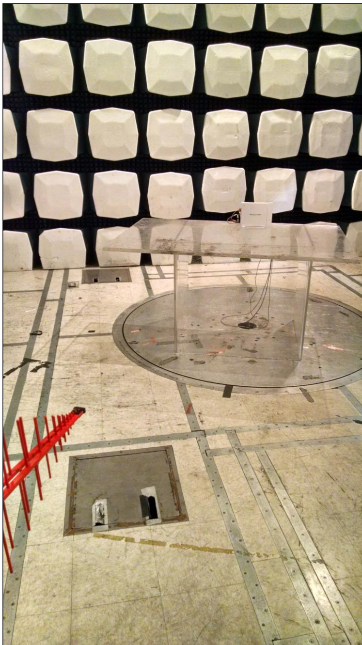
Photograph 1. Radiated Spurious Emissions, 30 MHz – 1 GHz, Test Setup
