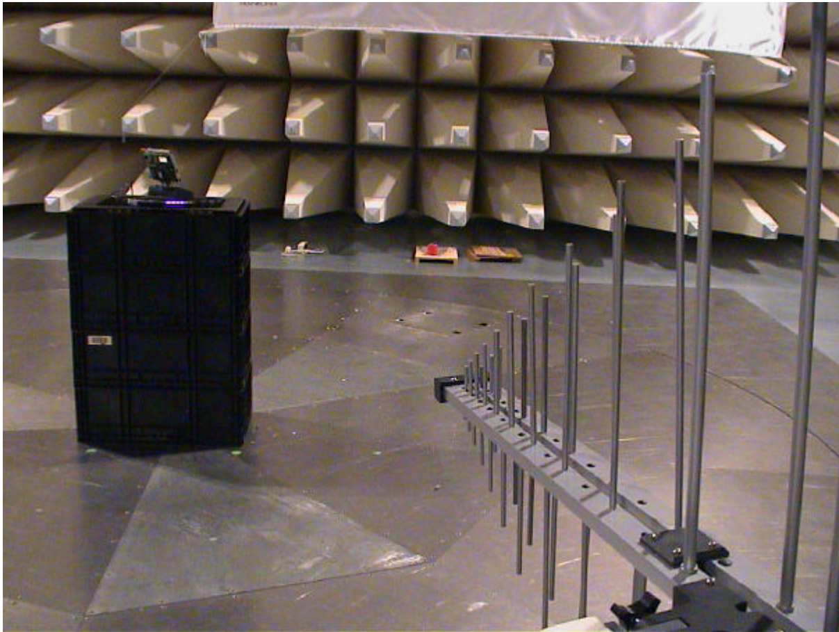
Fig. 2: Basic set-up for radiated and spurious emission; 30 MHz - 1 GHz
