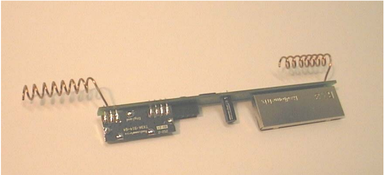
CS0188 touchCUE-SRF, RXTX module with antennas
