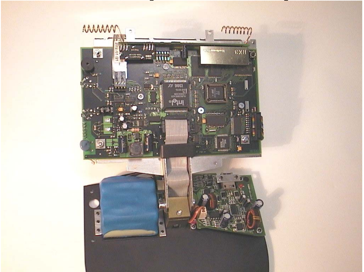
CS0188 touchCUE-SRF, configuration of mainboard, charger and RXTX.
