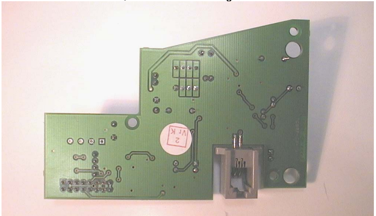
CS0188 touchCUE-SRF, bottom side of charger PCB
