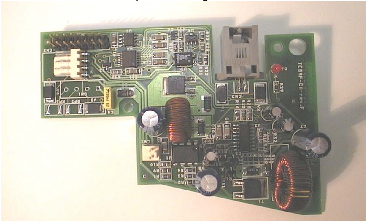
CS0188 touchCUE-SRF, top side of charger PCB
