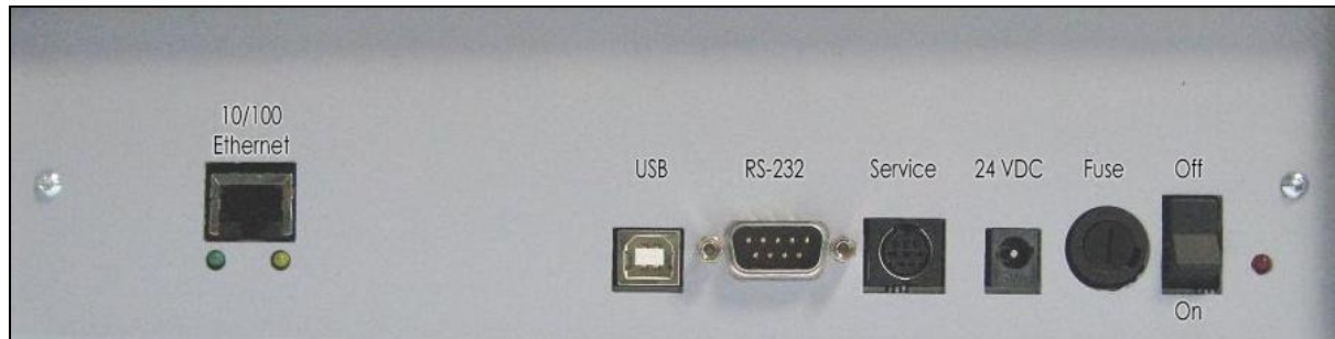
Figure 2: Rear panel
