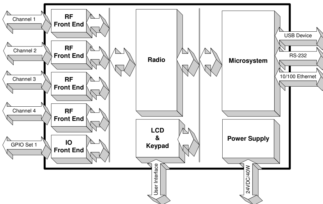
Figure 19: Medio L400 Architecture
