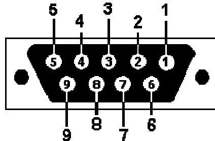
Figure 23: GPIO Connector (Female DB-9)
