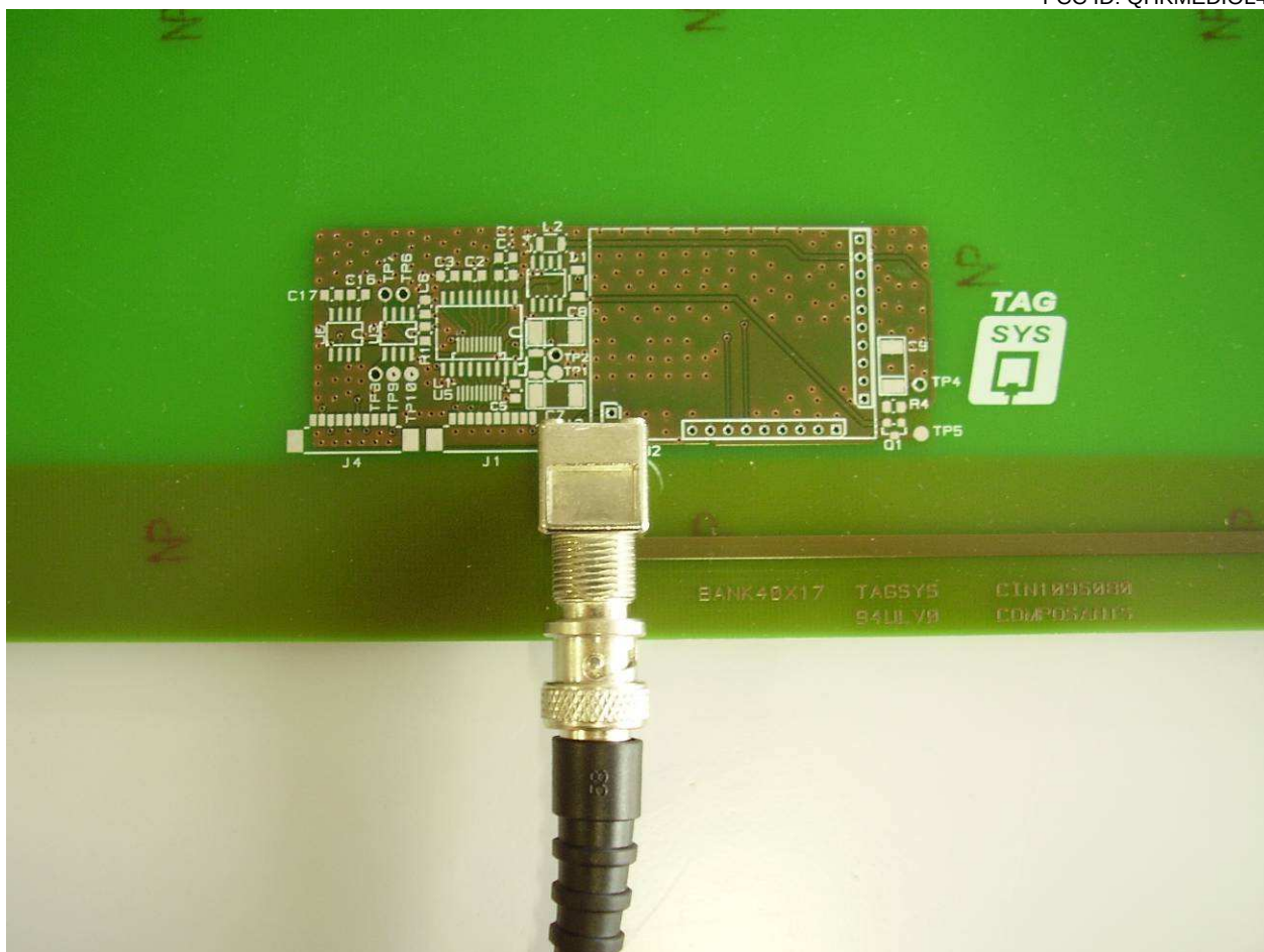
RF connector
