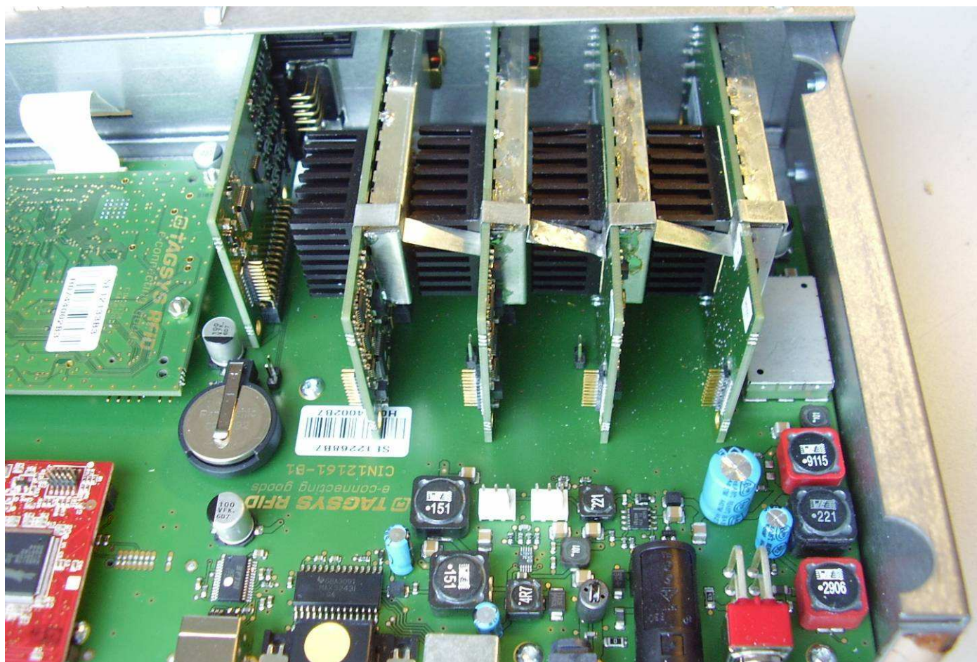
Detail view of RF boards
