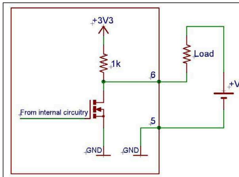
Figure 26: Connecting an external load to output #1
