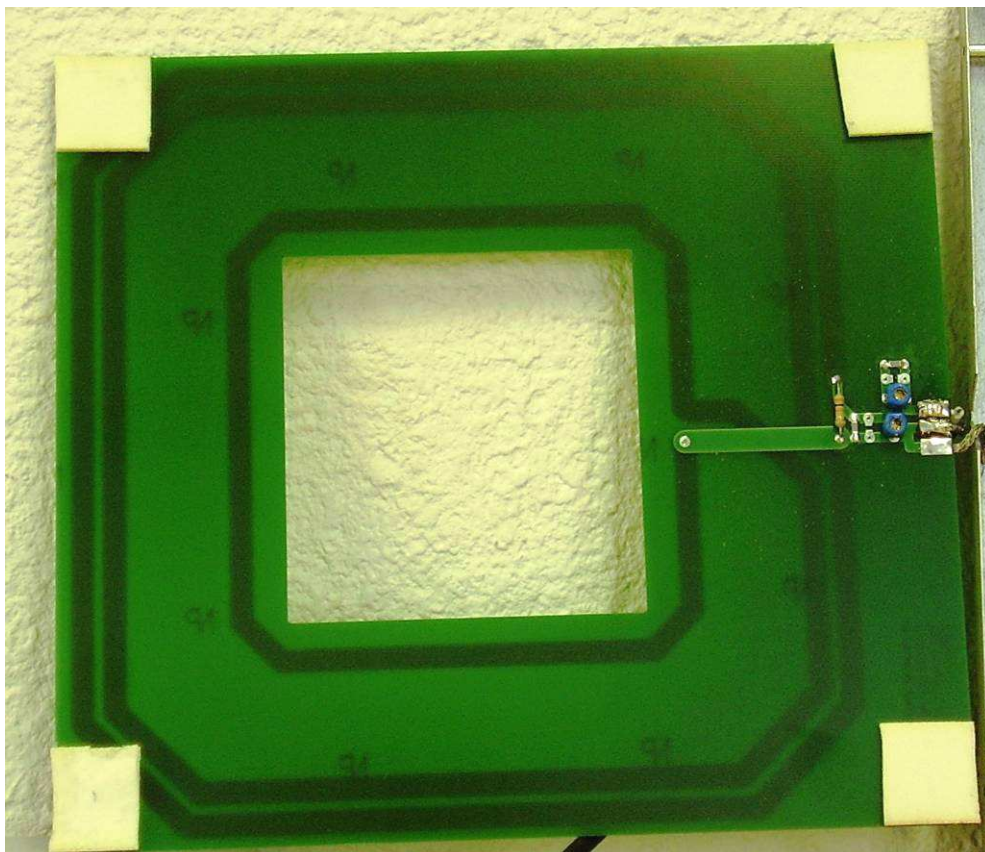
Antenna PCB
