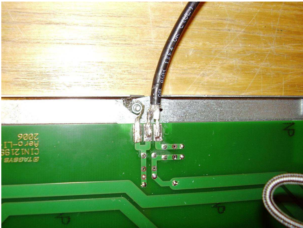
Detail view of the RF cable connection to PCB
