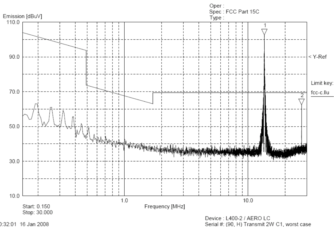
RADIATED EMISSION -TAGSYS RFID
