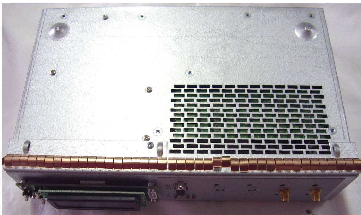
Lower metallic chassis (Under side, external housing removed)
