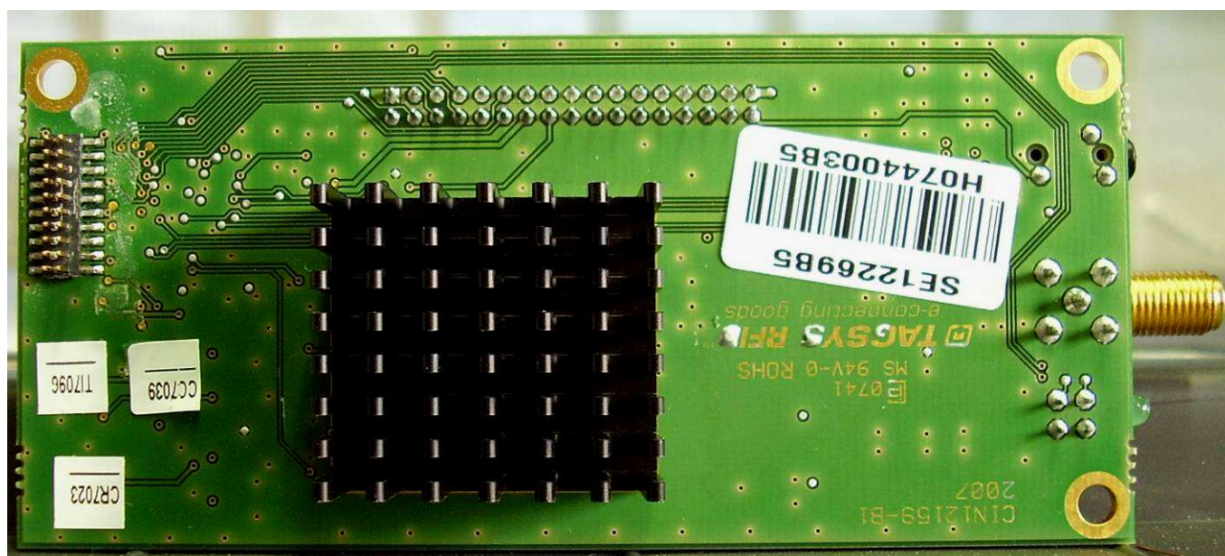
PCB of RF daughter board
