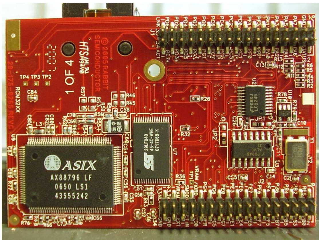
PCB of Ethernet board
