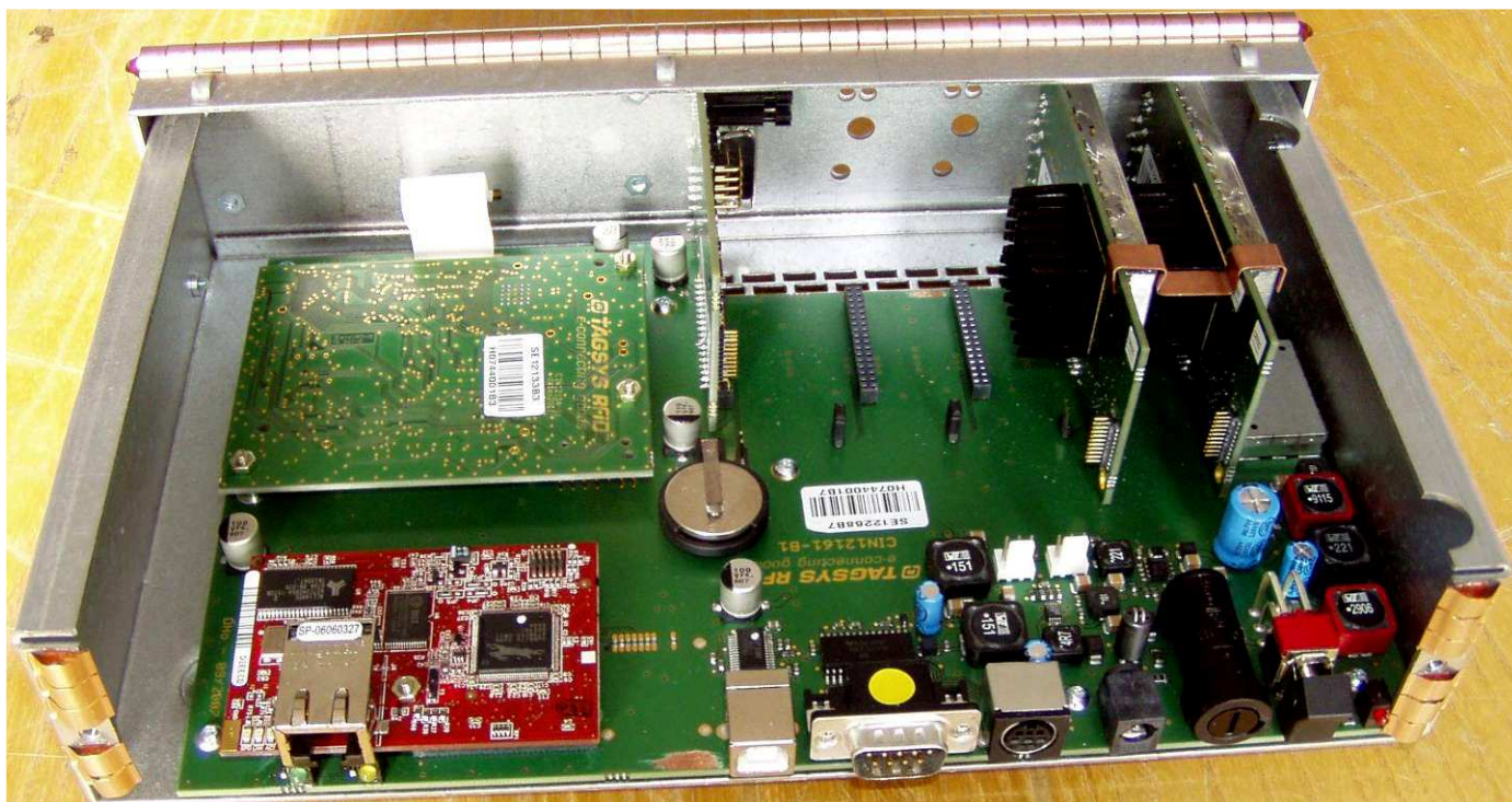
Cover removed (Rear side)
