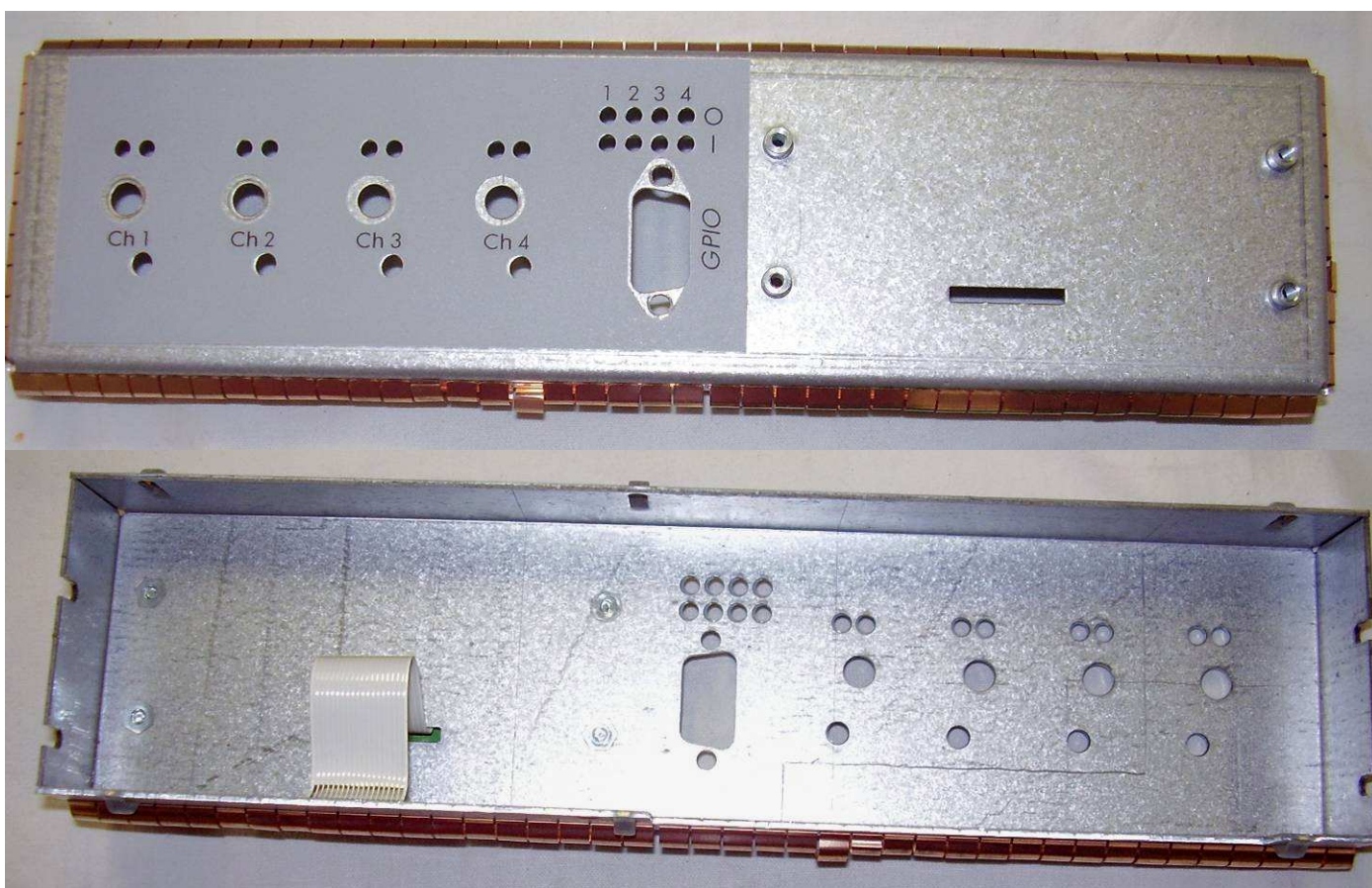
Detail view of front face
