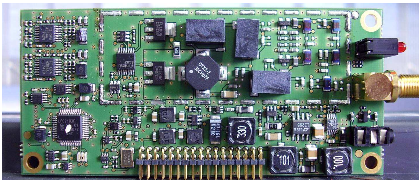
Metallic shield removed (RF board)
