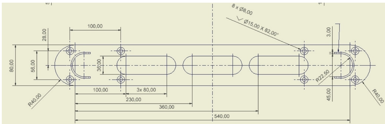
Figure 8: Pedestal Mounting Base Dimensions
