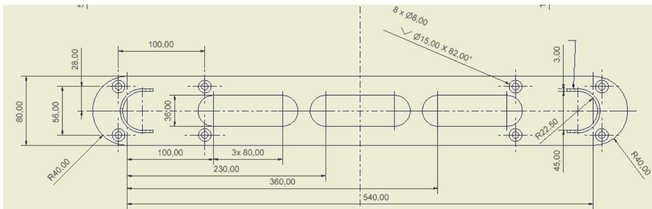
Figure 30: Mechanical Dimensions of Pedestal Base Fixing Plate
