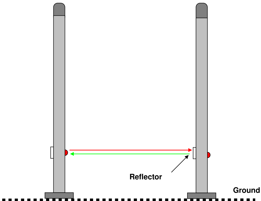
Figure 6: Side view of correct L-SP3 installation
