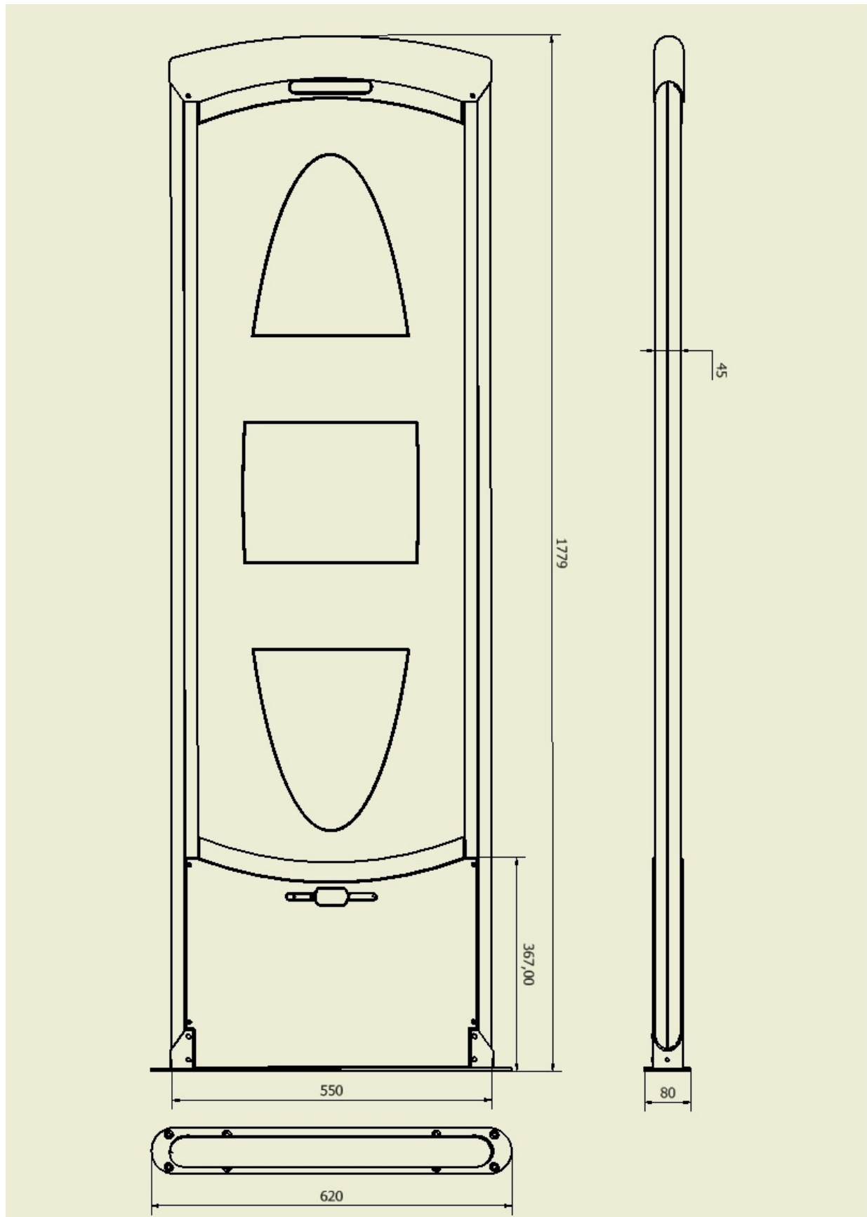
Figure 31: Outer Dimensions of LSP3 Panel
