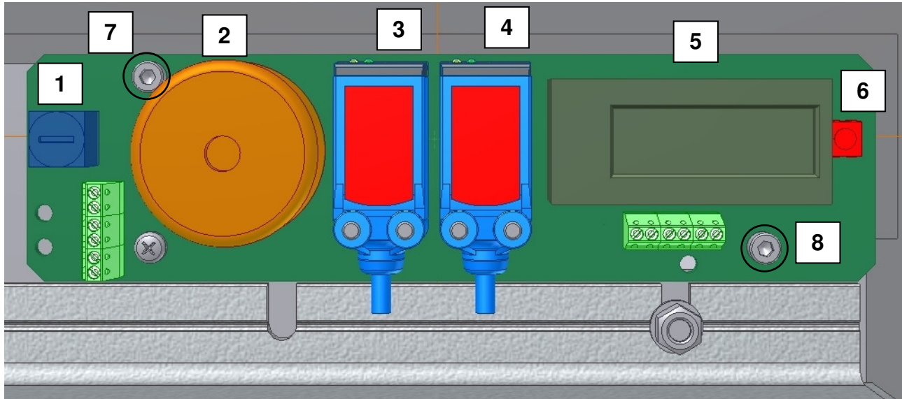
Figure 7: Beam Crossing Detection Cells and Adjustment screws
