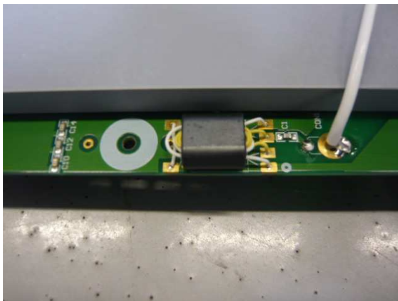
Detail views of antenna
