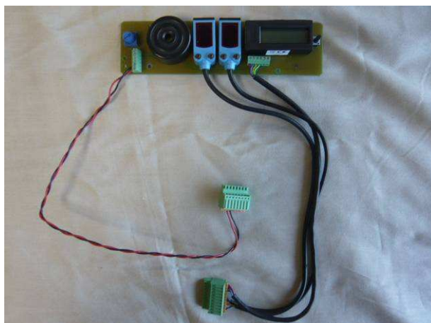
Counter and warning device
