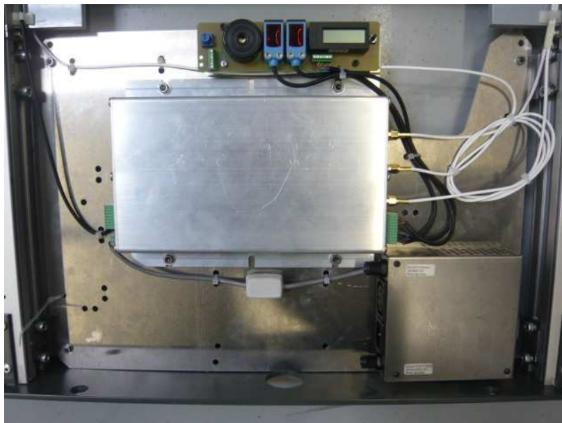
Antenna connection to the reader box
