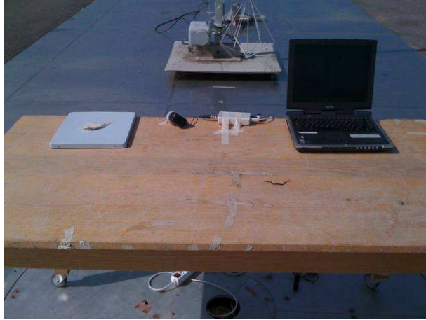
Radiated setup – LSA4 SHD configuration
