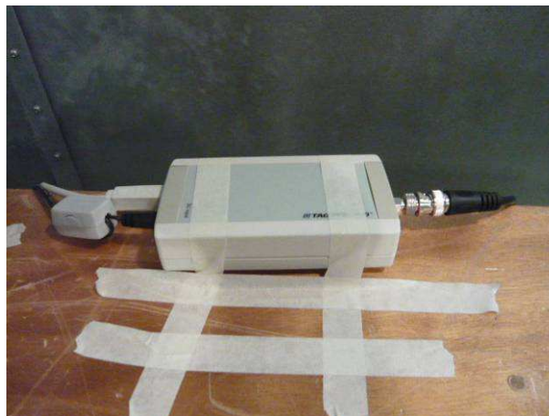
Conducted setup – LSA4 SHD Antenna
