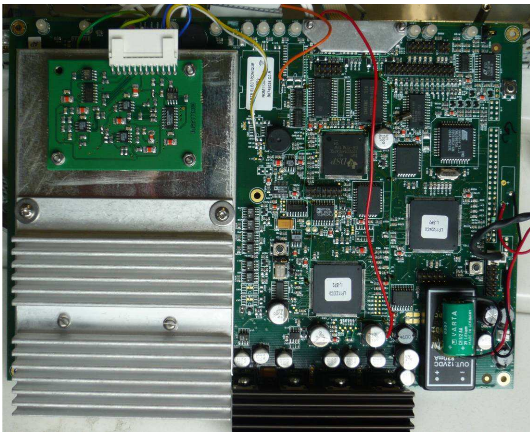
Electronic board
