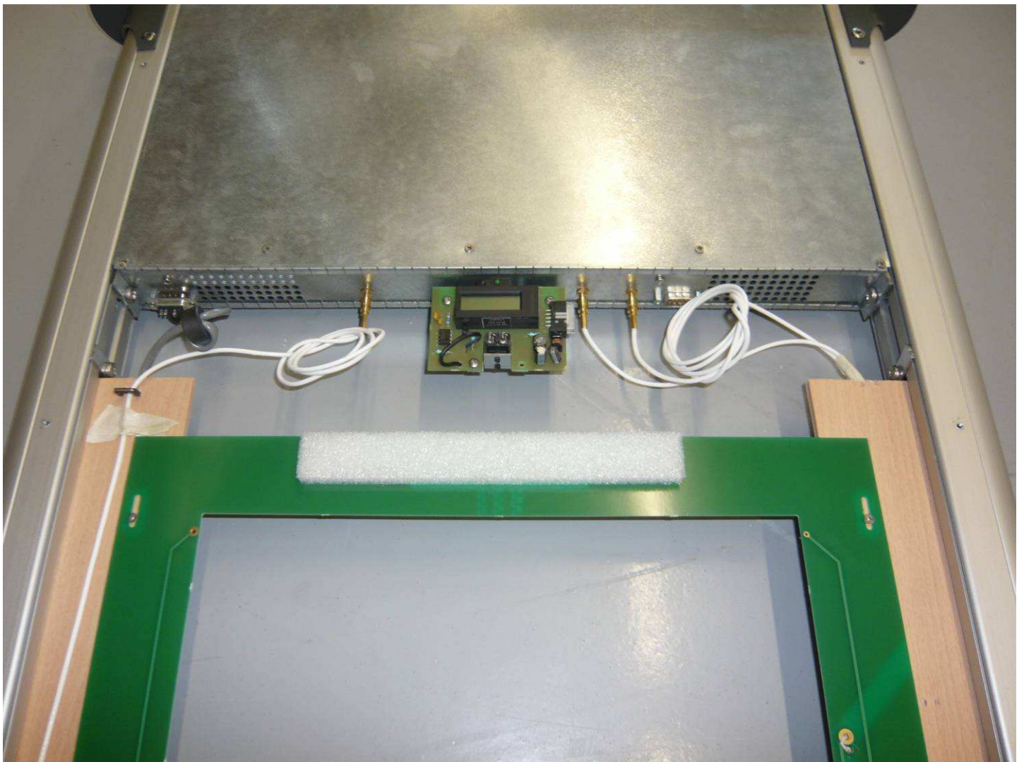
Antenna connection to the reader box
