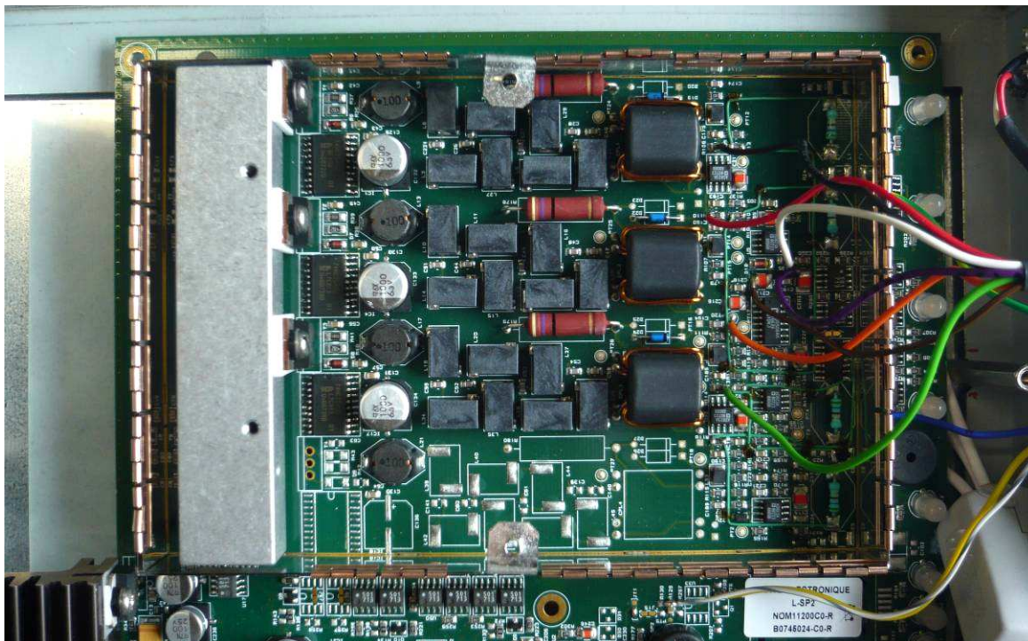
RF module (Shielding cover removed)
