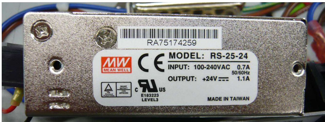
Power supply unit
