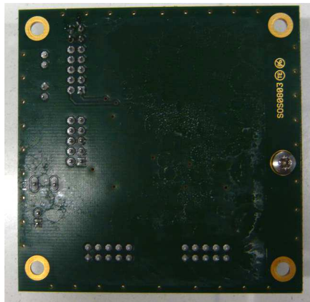
Communication board
