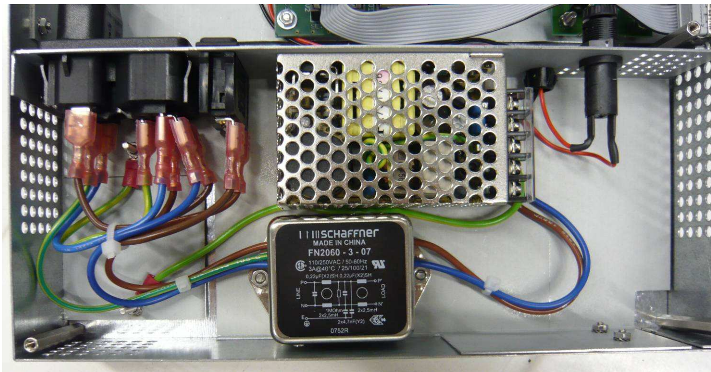
Power supply unit
