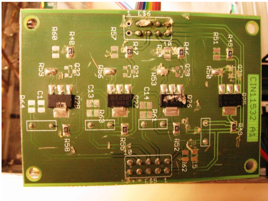
Bottom View (against internal wall of casing) of L200 Antenna Tuning Solid State Switch Card Drive
