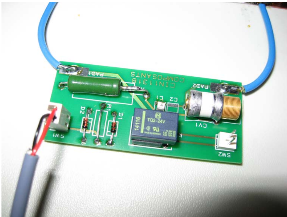
Antenna Tuning Board alone
