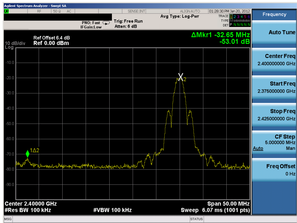
Plot 6-8. Band Edge Plot (802.15.4 – Ch. 12)
