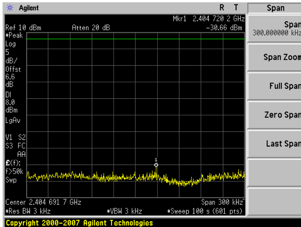
Plot 6-4. Power Spectral Density Plot (802.15.4 – Ch. 11)
