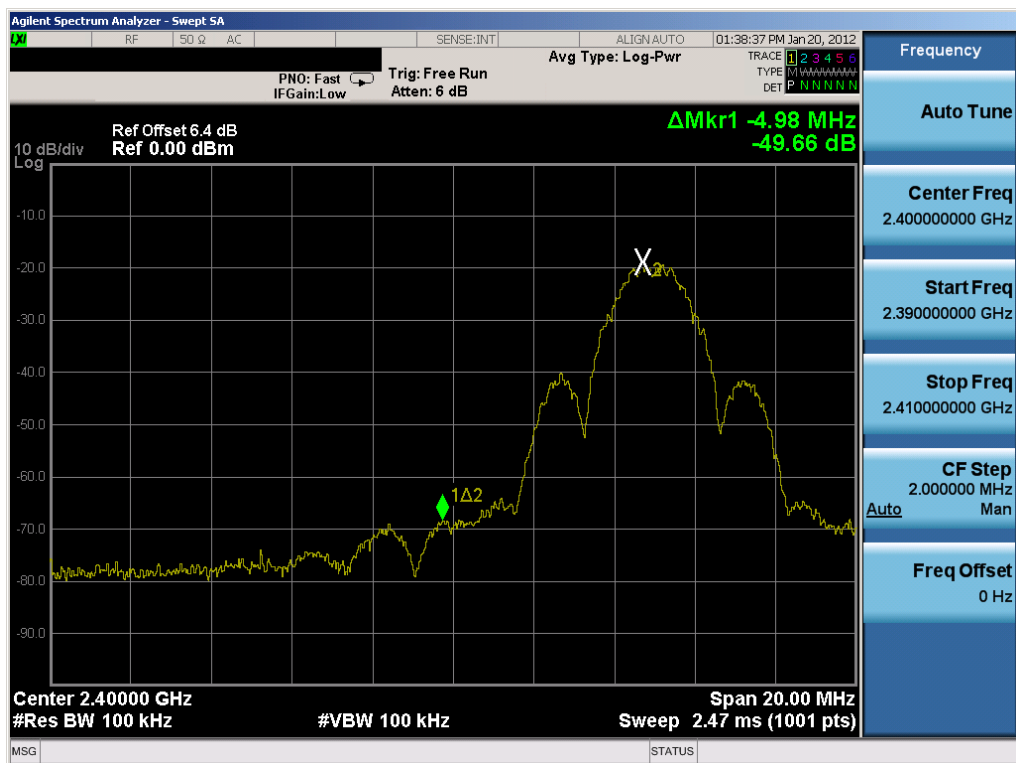
Plot 6-7. Band Edge Plot (802.15.4 – Ch. 11)
