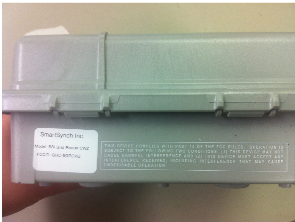
SSI GridRouter CWZ FCC ID Label Placement
