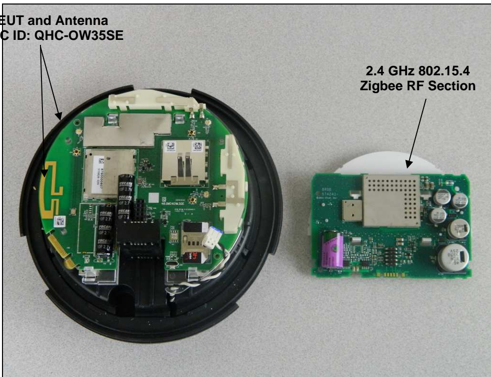
Figure 4: Internal Photo
