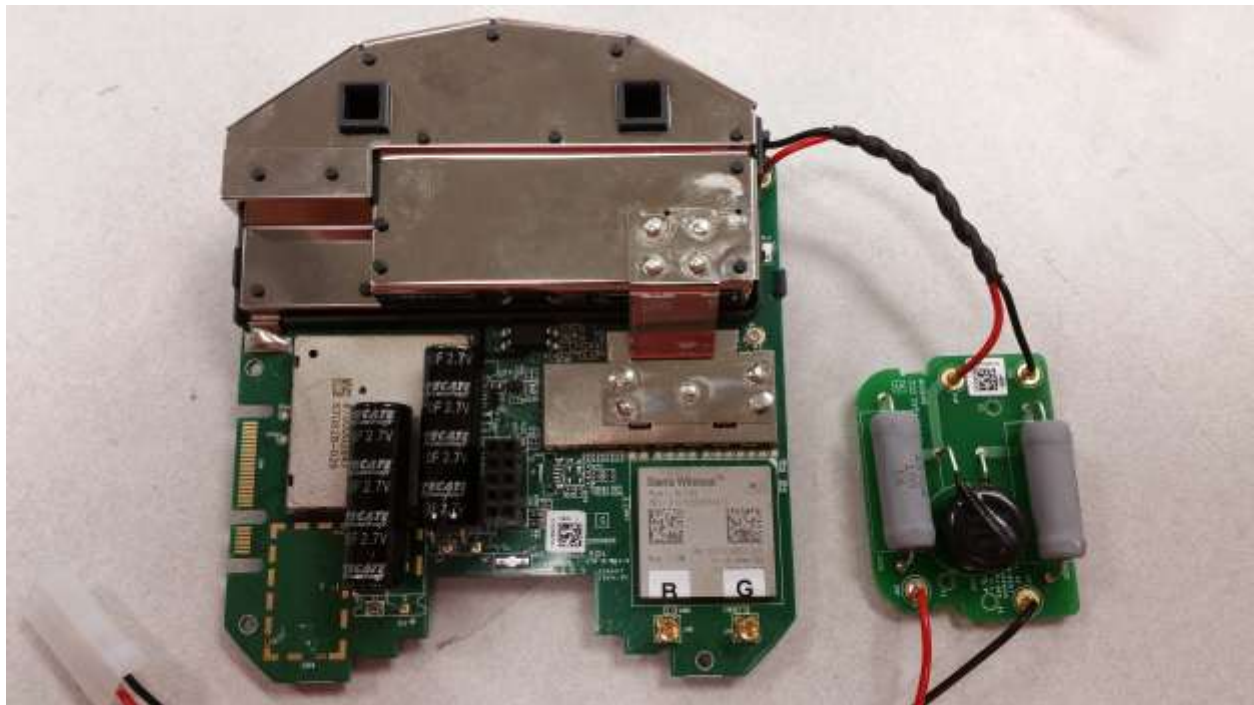
MODULE 574161 FRONT WITH SHIELDS
