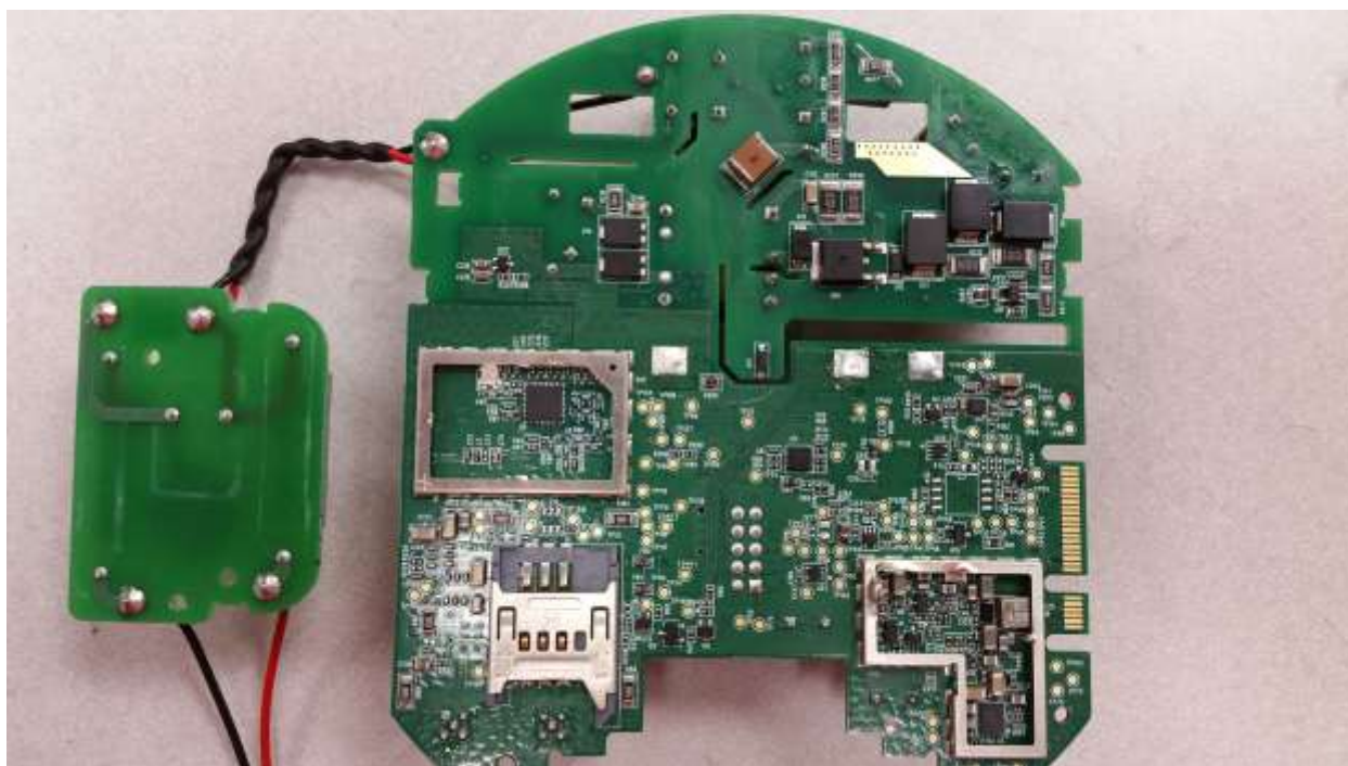
MODULE 574161 BACK WITH SHIELDS REMOVED
