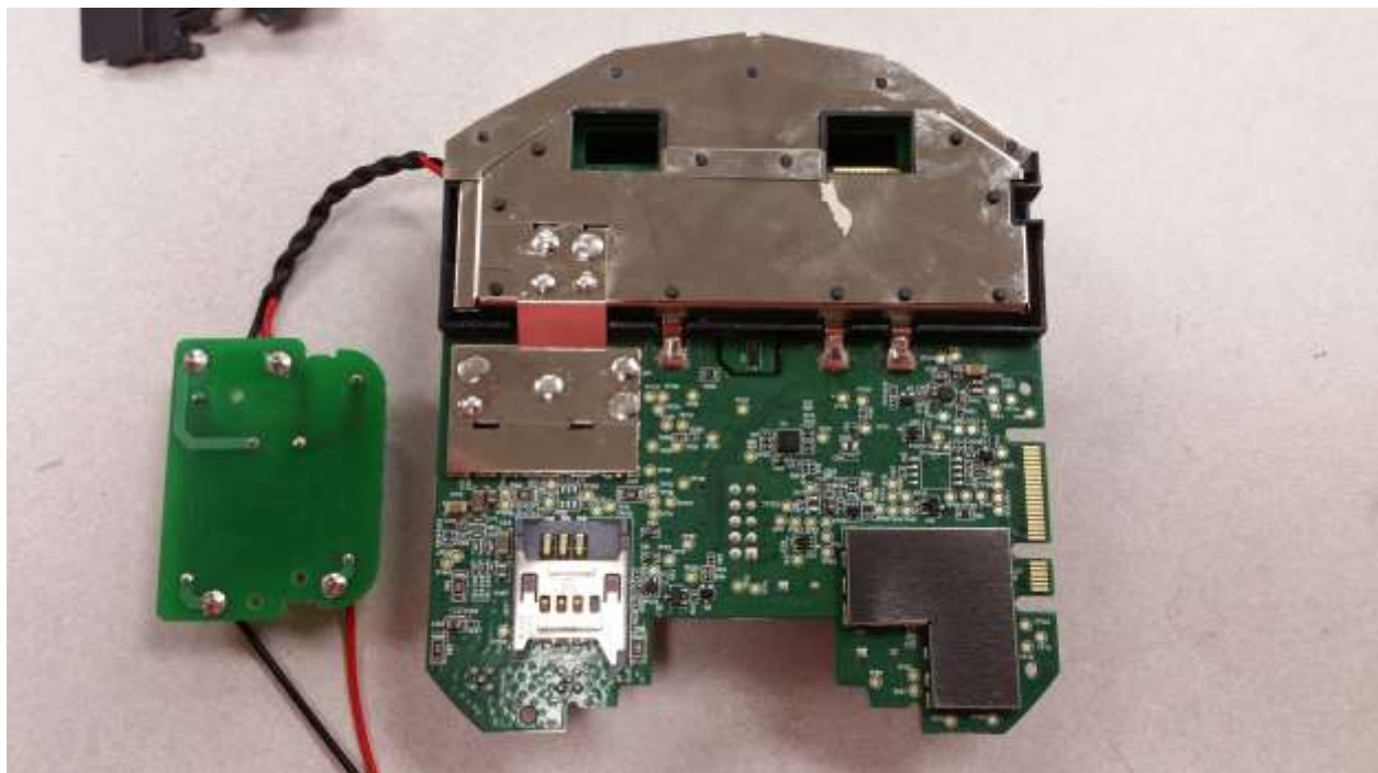
MODULE 574161 BACK WITH SHIELDS
