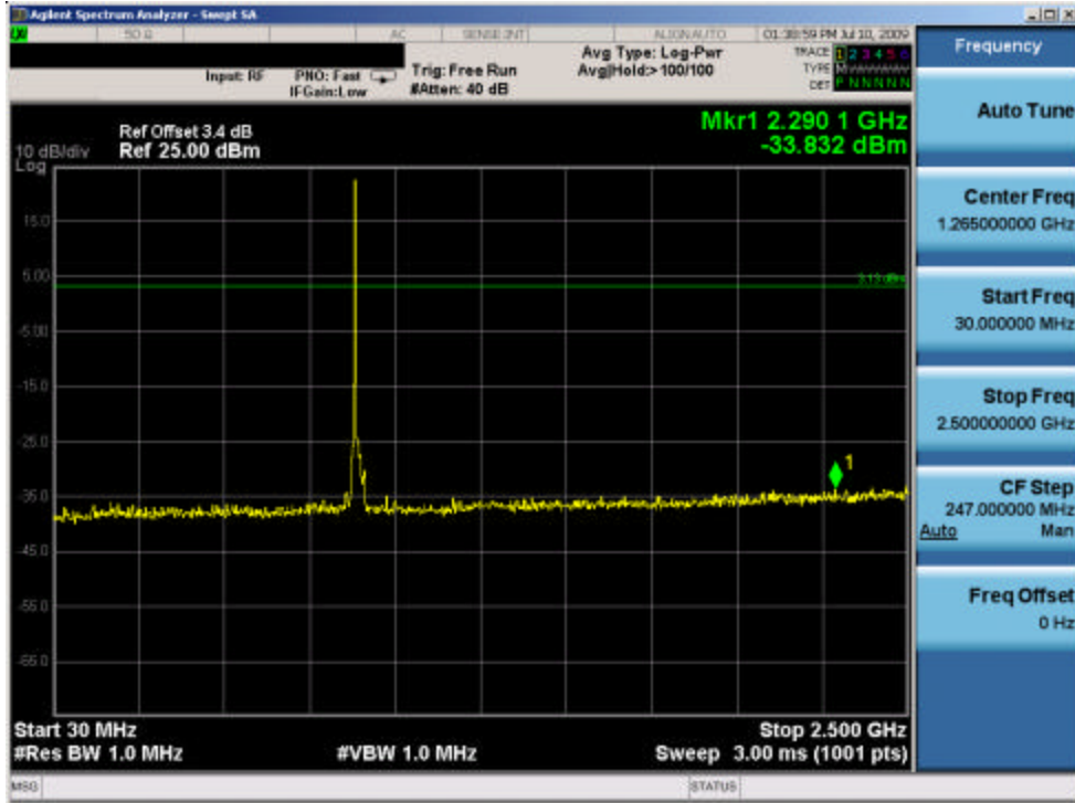
Plot 6-15. Conducted Spurious Plot (Ch. 0)
