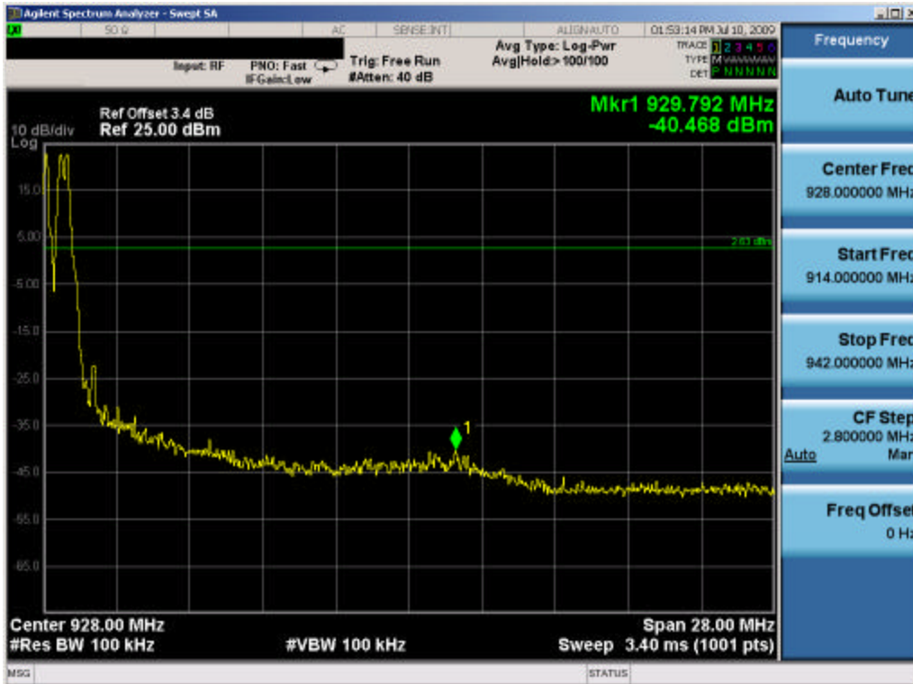
Plot 6-10. Upper Band Edge Plot (Hopping Mode – Ch. 31)
