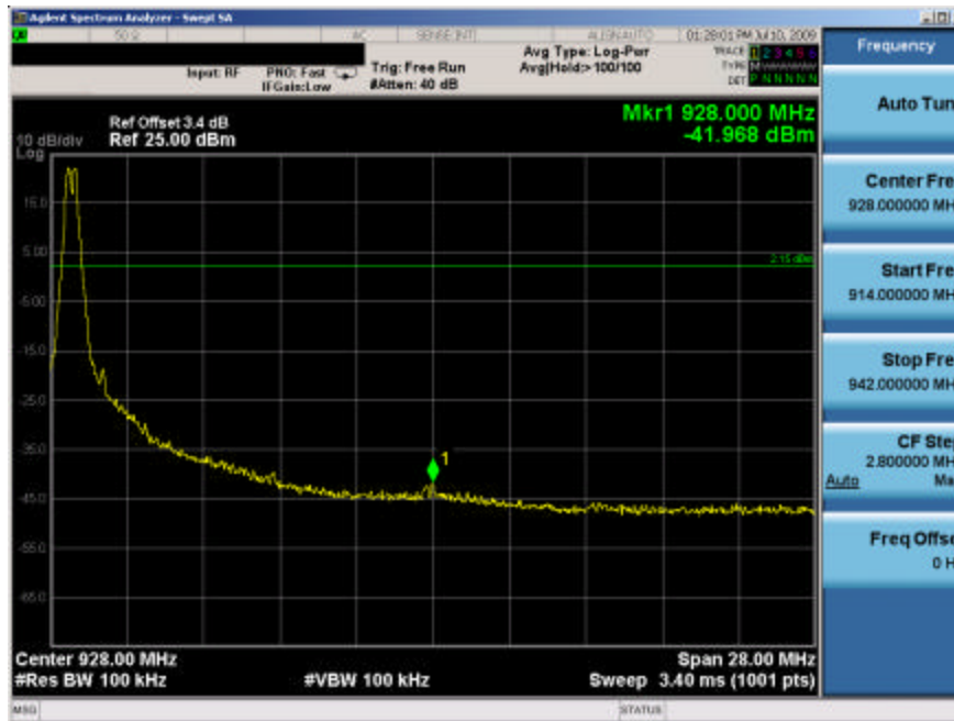
Plot 6-8. Upper Band Edge Plot (Ch. 31)
