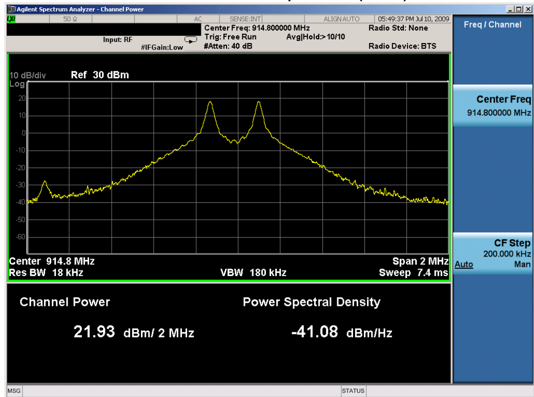
Plot 6-6. Conducted Output Power (Ch. 31)
