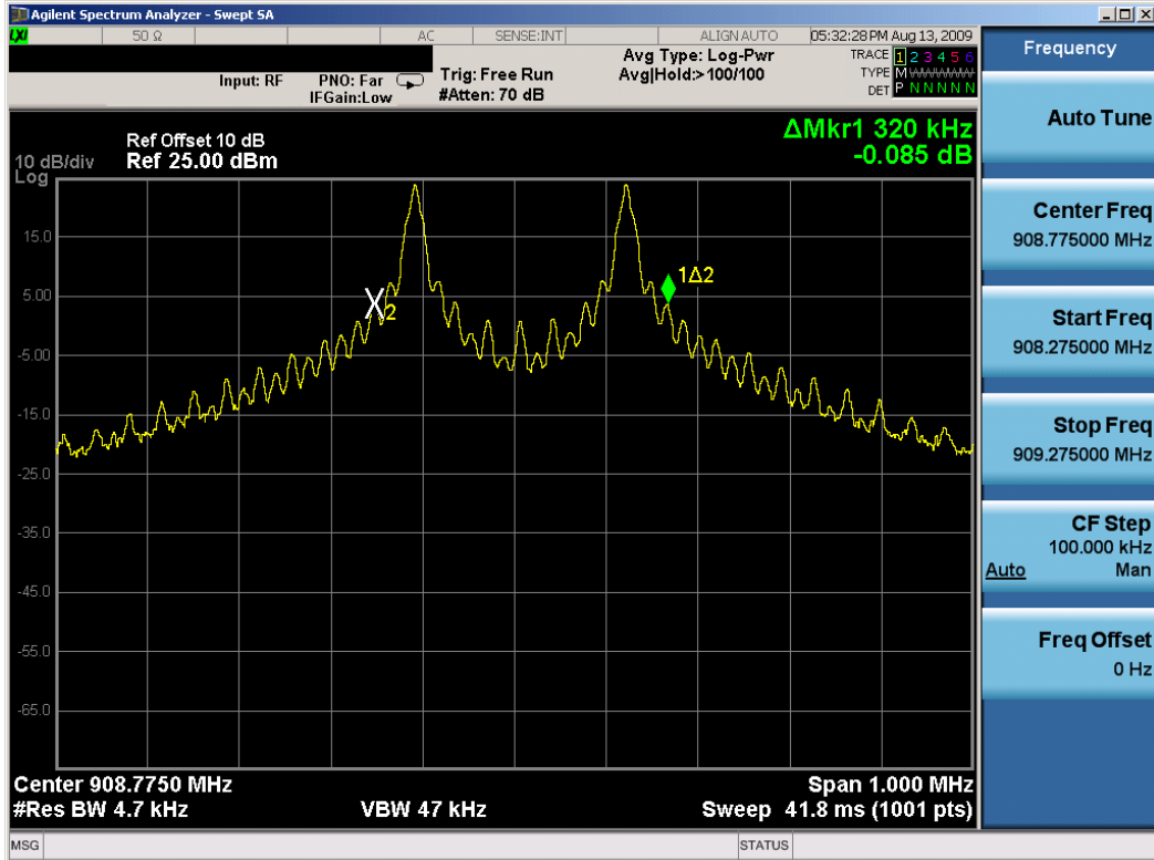
Plot 6-2. 20dB Bandwidth Plot (Ch. 16)
