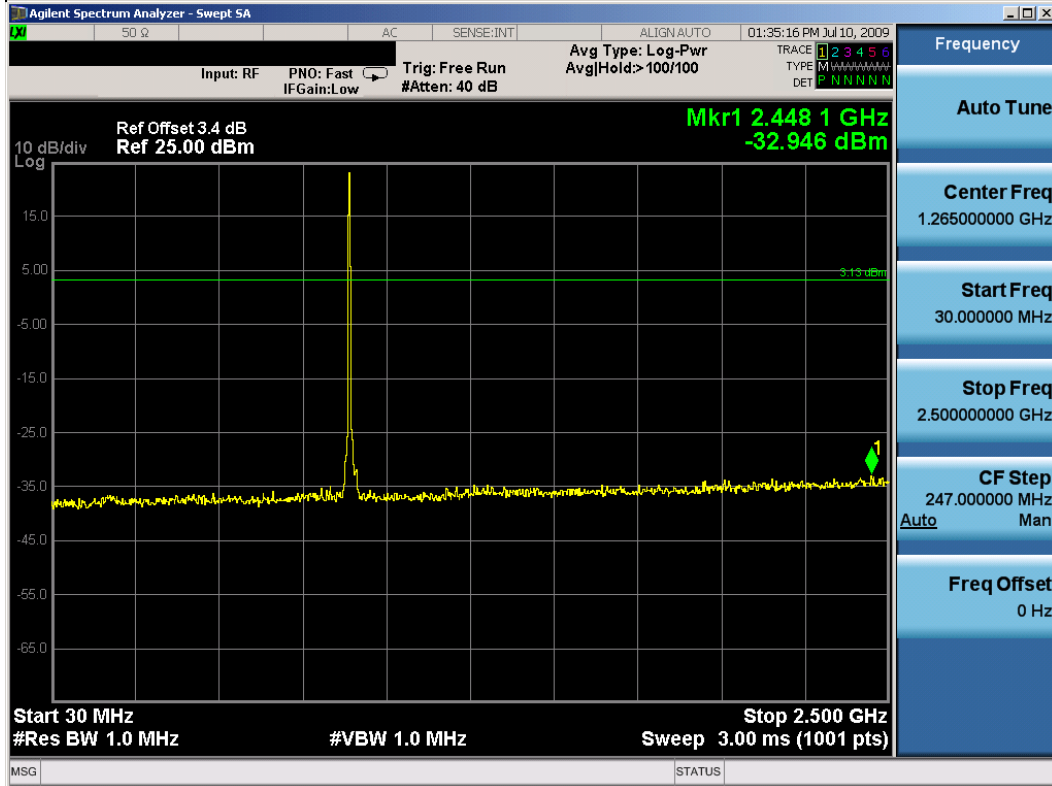
Plot 6-17. Conducted Spurious Plot (Ch. 16)
