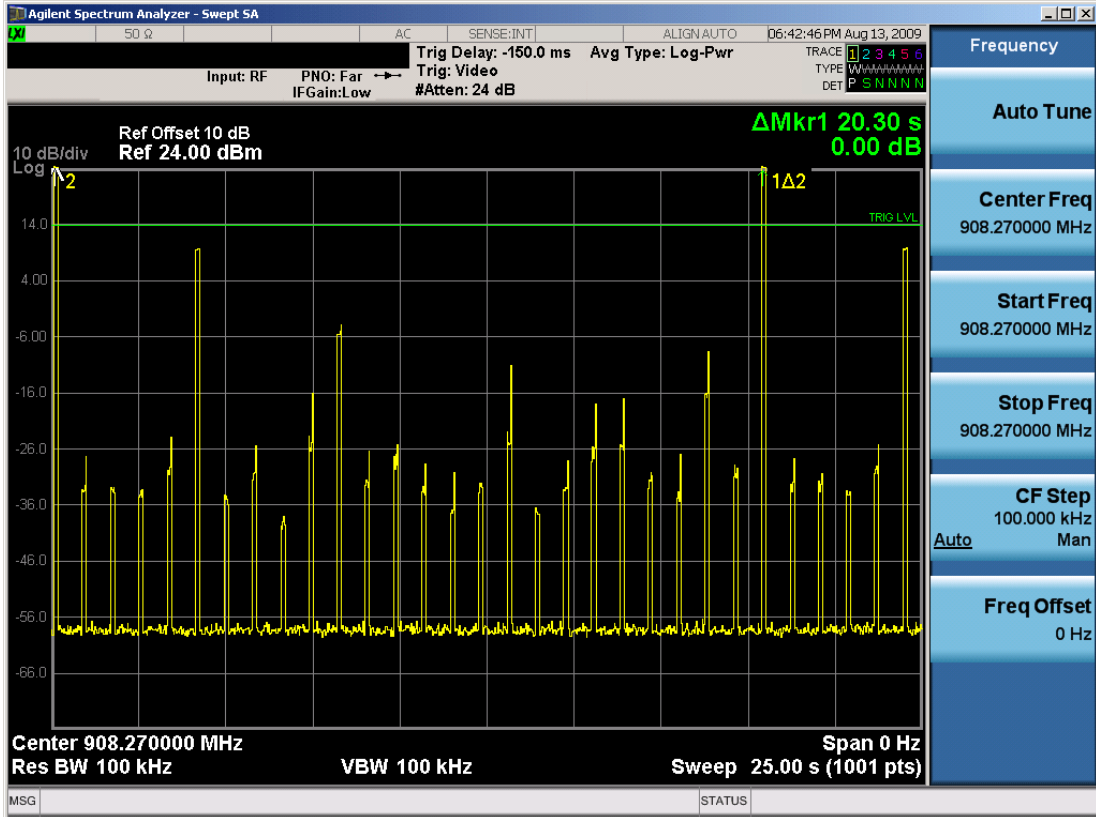
Plot 6-13. Time of Occupancy Plot
