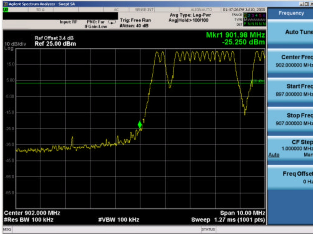
Plot 6-9. Lower Band Edge Plot (Hopping Mode – Ch. 0)
