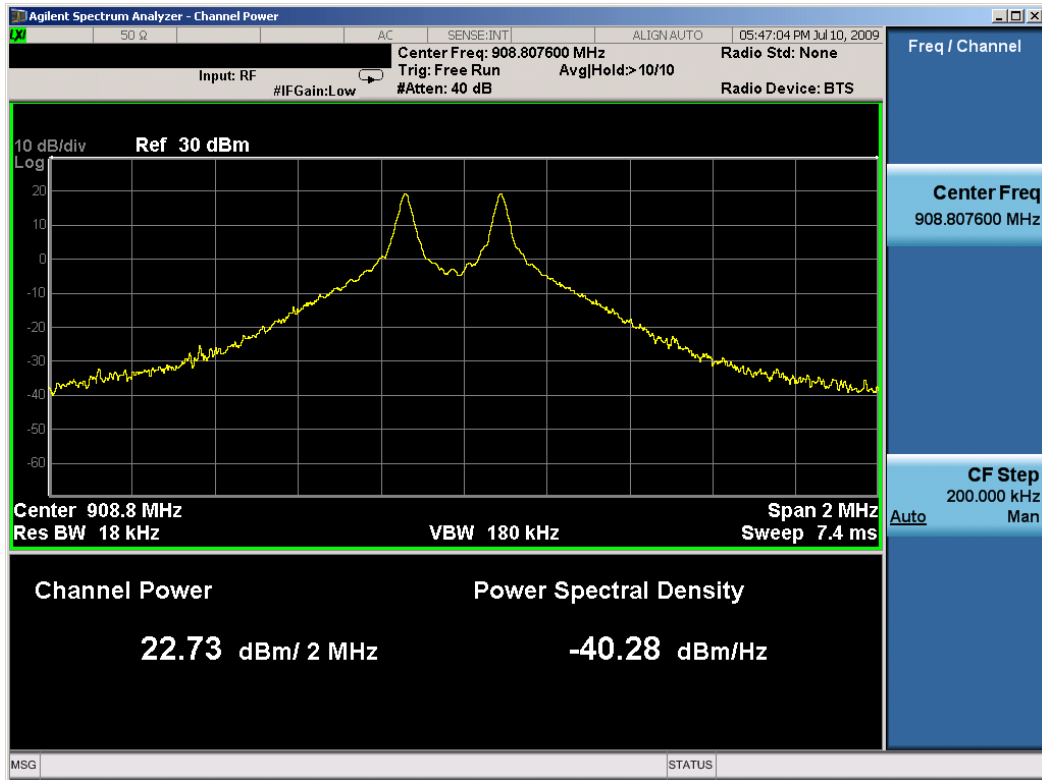
Plot 6-5. Conducted Output Power (Ch. 16)
