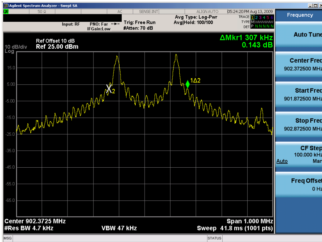
Plot 6-1. 20dB Bandwidth Plot (Ch. 0)
