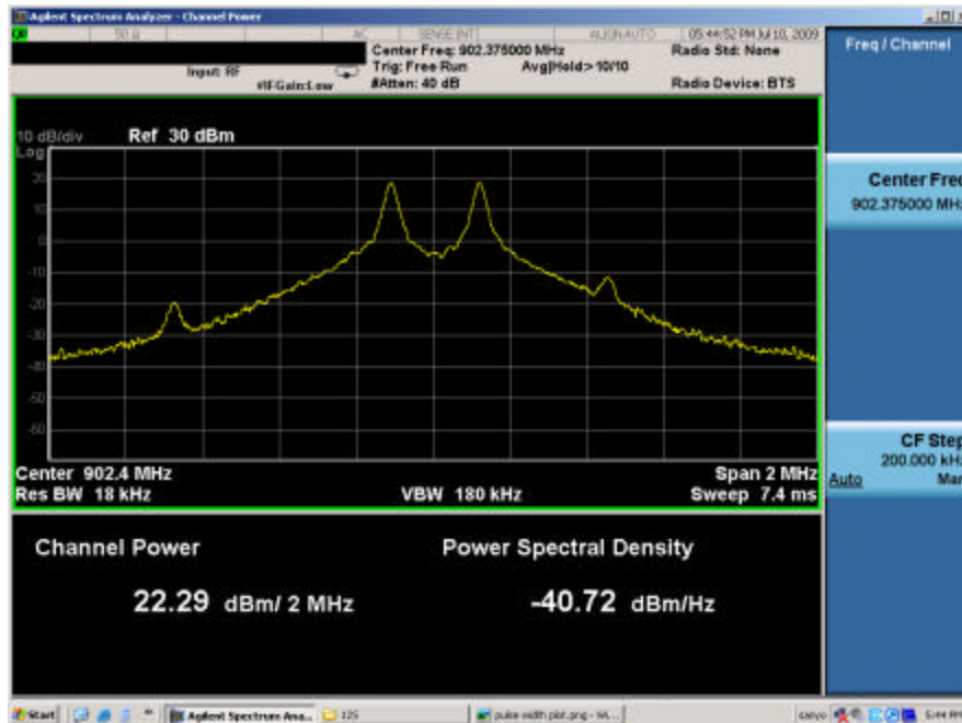
Plot 6-4. Conducted Output Power (Ch. 0)
