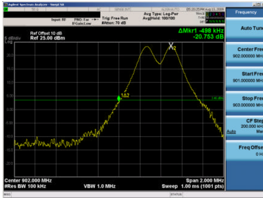
Plot 6-7. Lower Band Edge Plot (Ch. 0)
