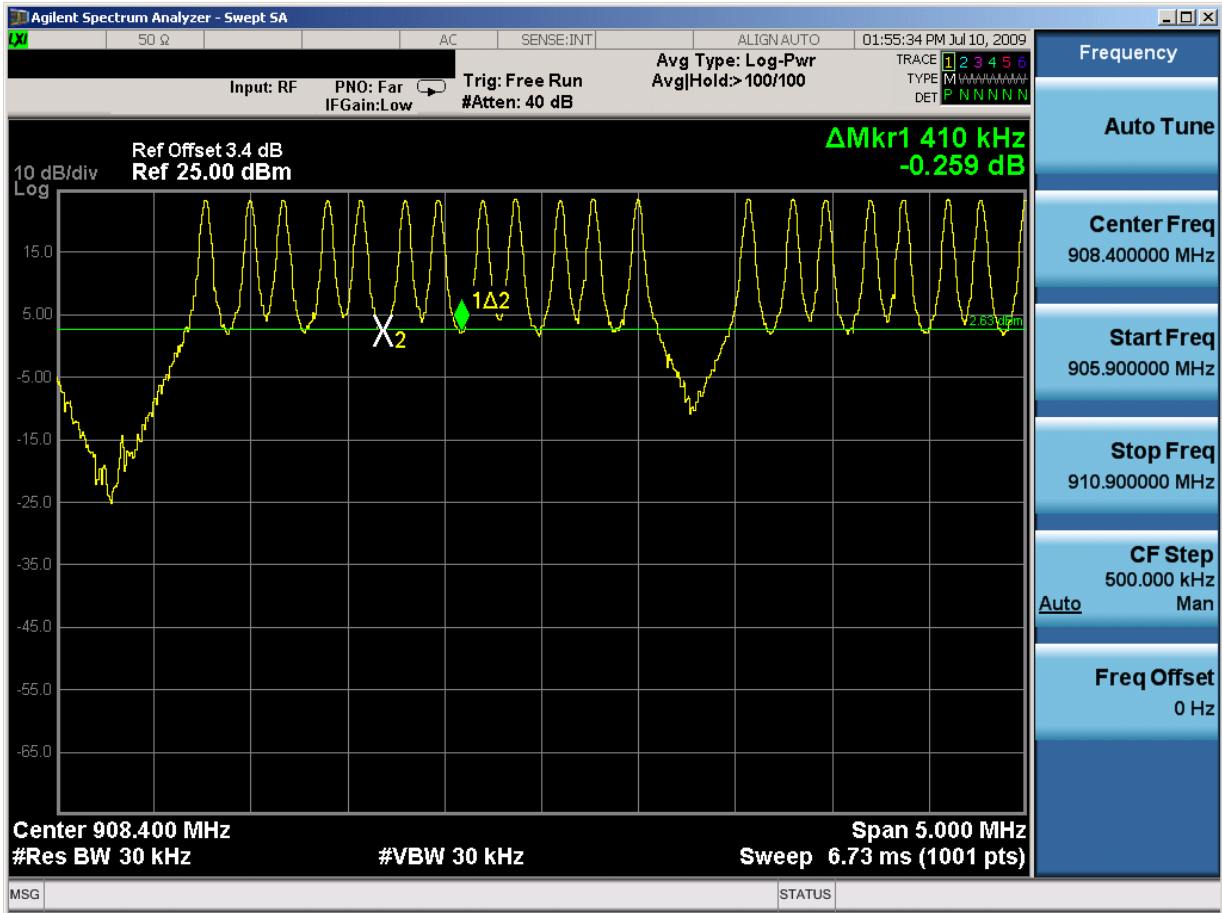
Plot 6-11. Channel Spacing Plot (Hopping Mode)
