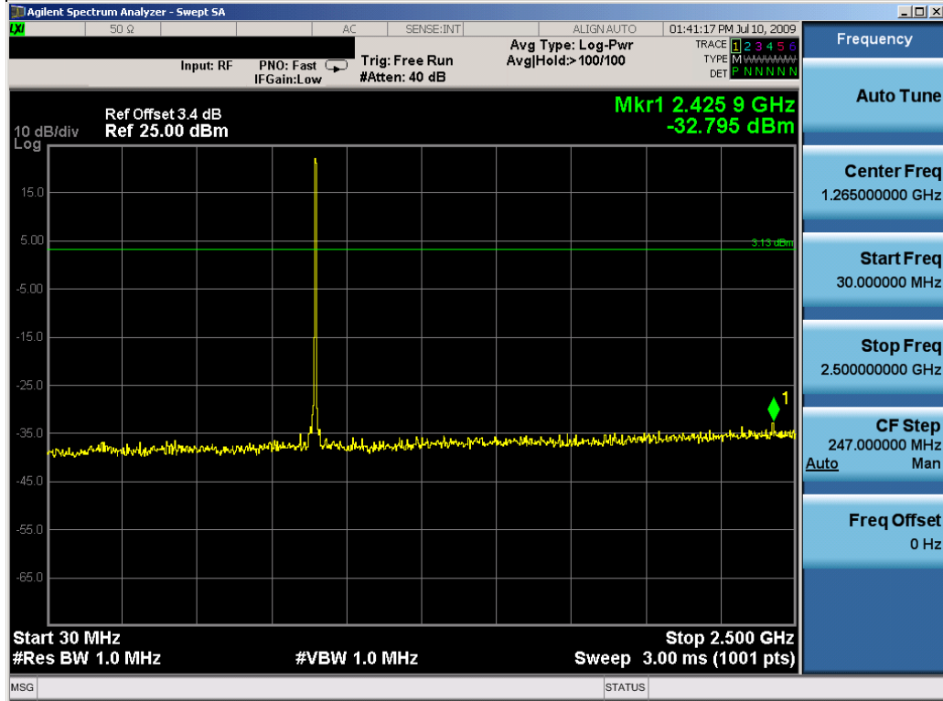
Plot 6-19. Conducted Spurious Plot (Ch. 31)
