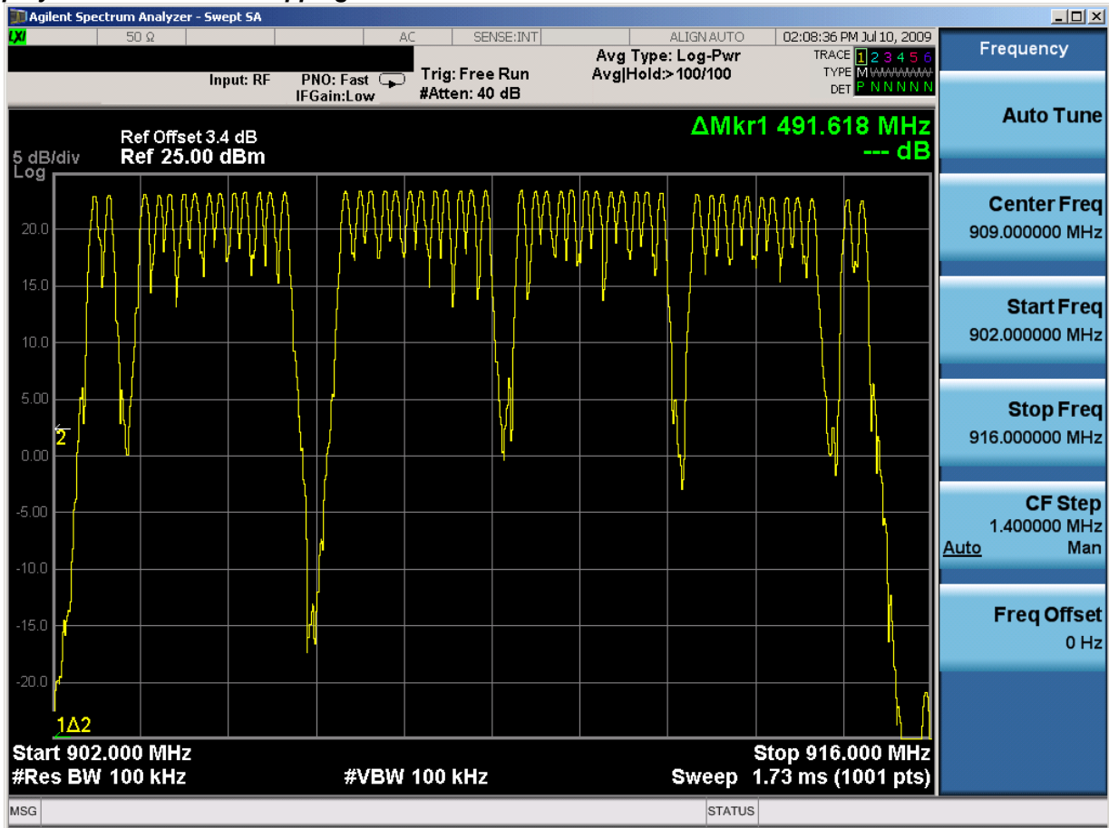
Plot 6-14. 900MHz Spectrum Channel Hopping Plot
