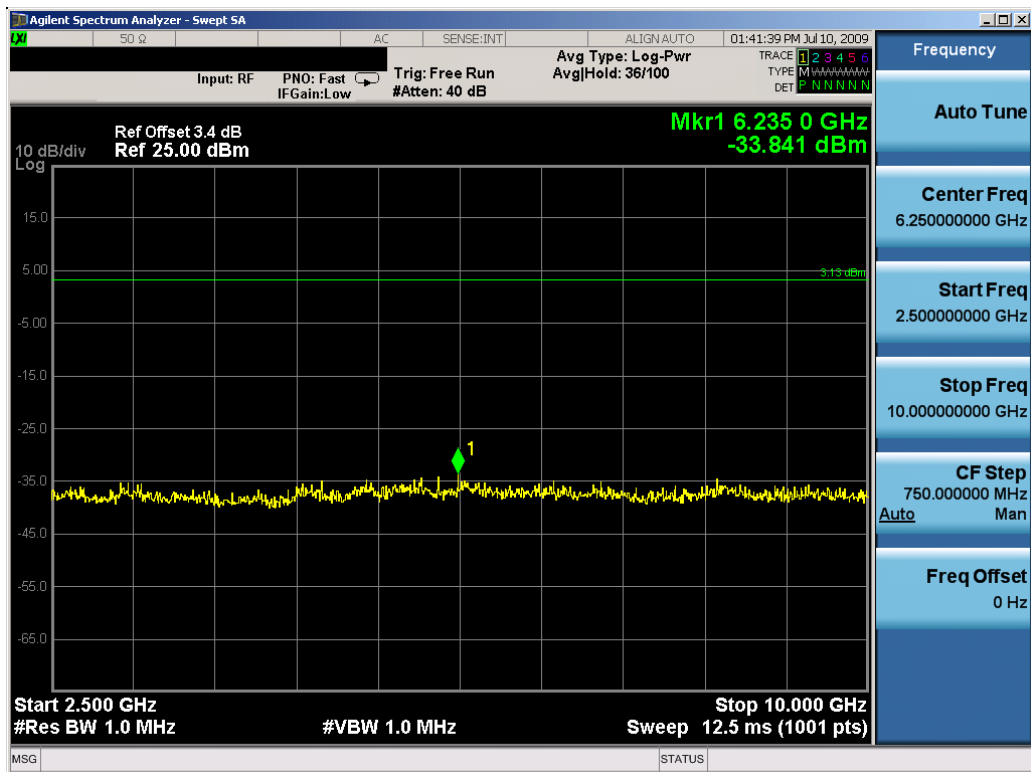
Plot 6-20. Conducted Spurious Plot (Ch. 31)
