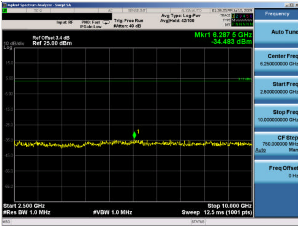
Plot 6-16. Conducted Spurious Plot (Ch. 0)
