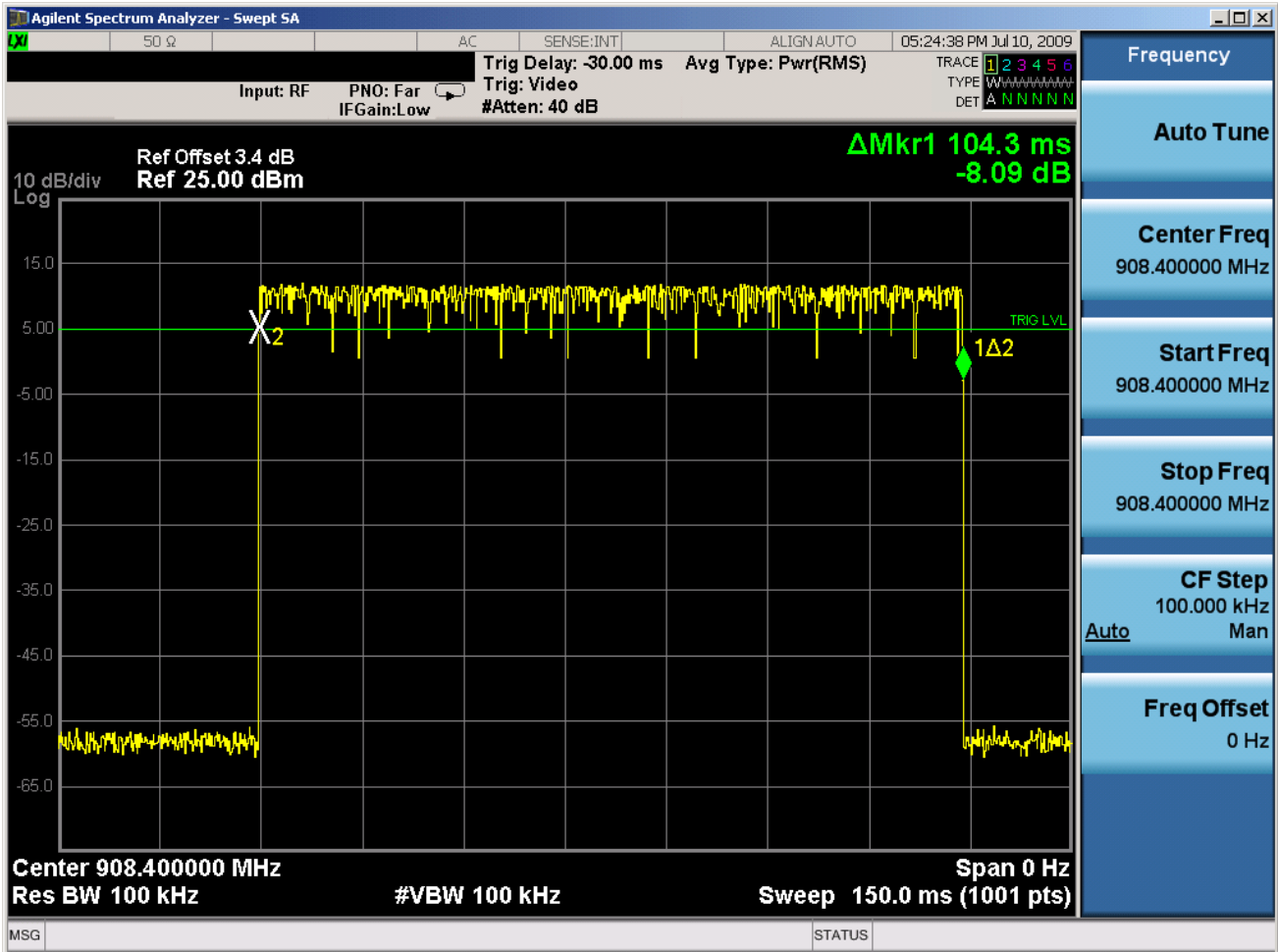
Plot 6-12. Pulse Width Plot
