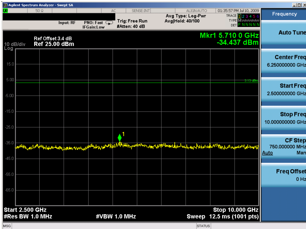
Plot 6-18. Conducted Spurious Plot (Ch. 16)
