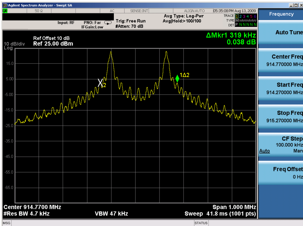
Plot 6-3. 20dB Bandwidth Plot (Ch. 31)
