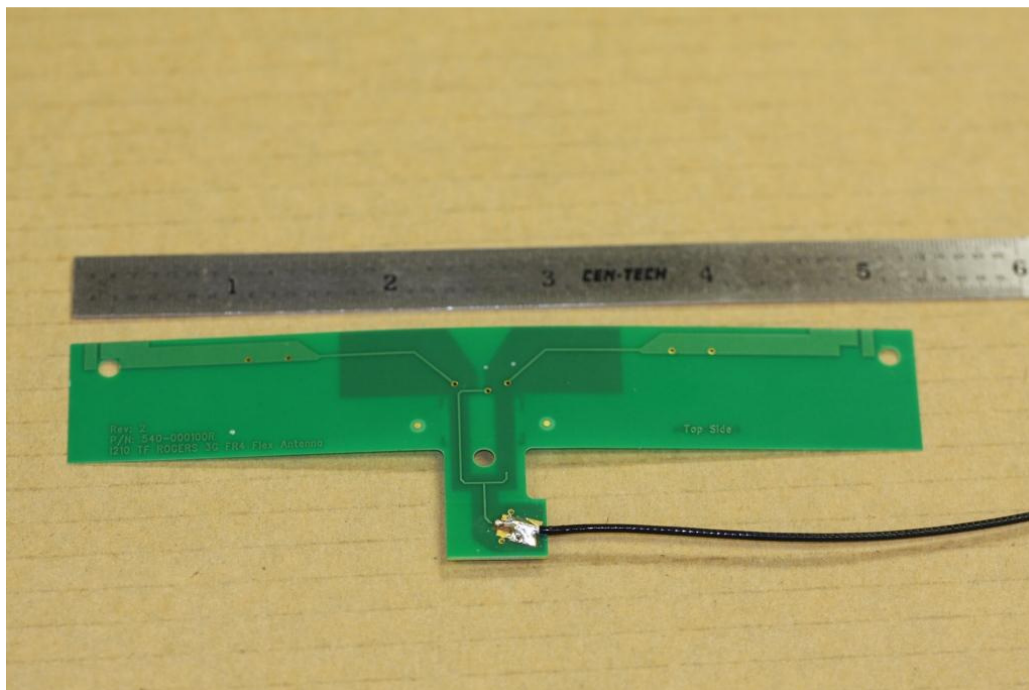
I210 3G WAN ANTENNA – RIBBON DIPOLE LENGTH
