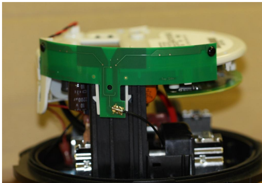
I210 3G WAN ANTENNA POSITION
