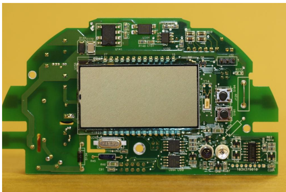
I210 3G METER REGISTER – FRONT
