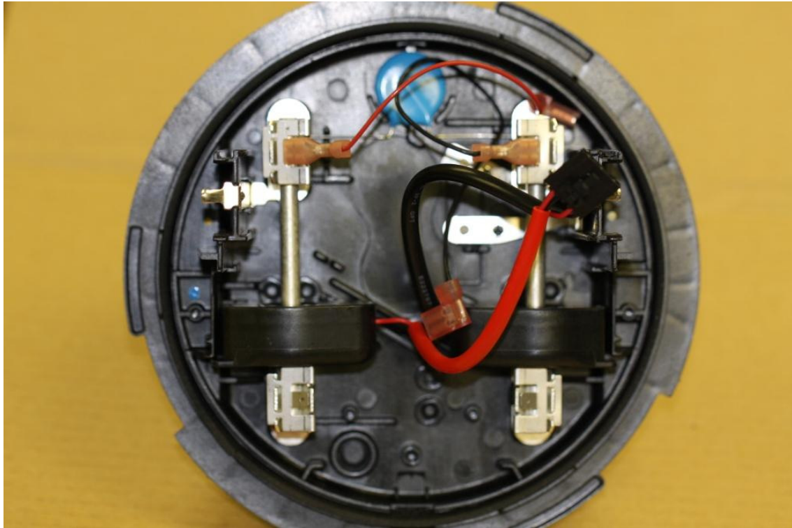
I210 3G METER BASE – INTERNAL
