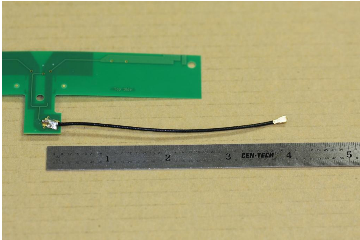
I210 3G WAN ANTENNA RF CABLE
