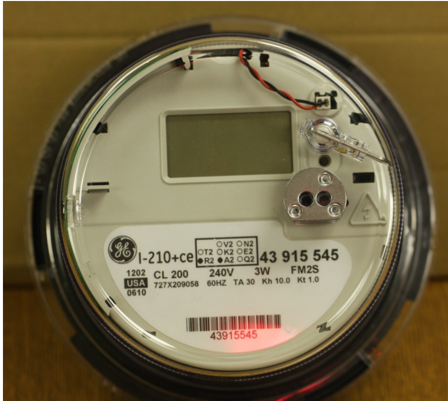
I210 3G METER ASSEMBLED
