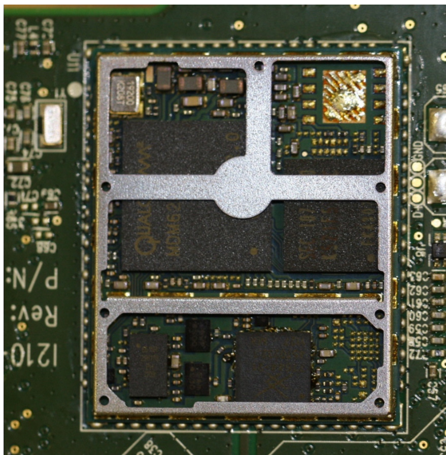
I210 3G SL8081 – SHIELD REMOVED
