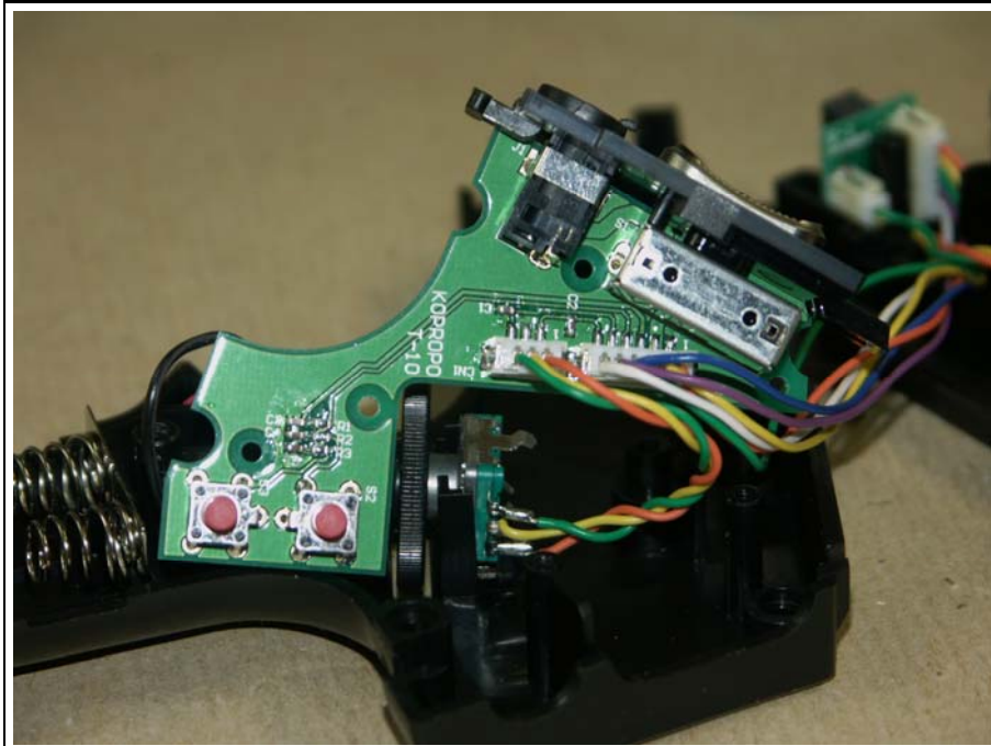
GRIP UNIT
