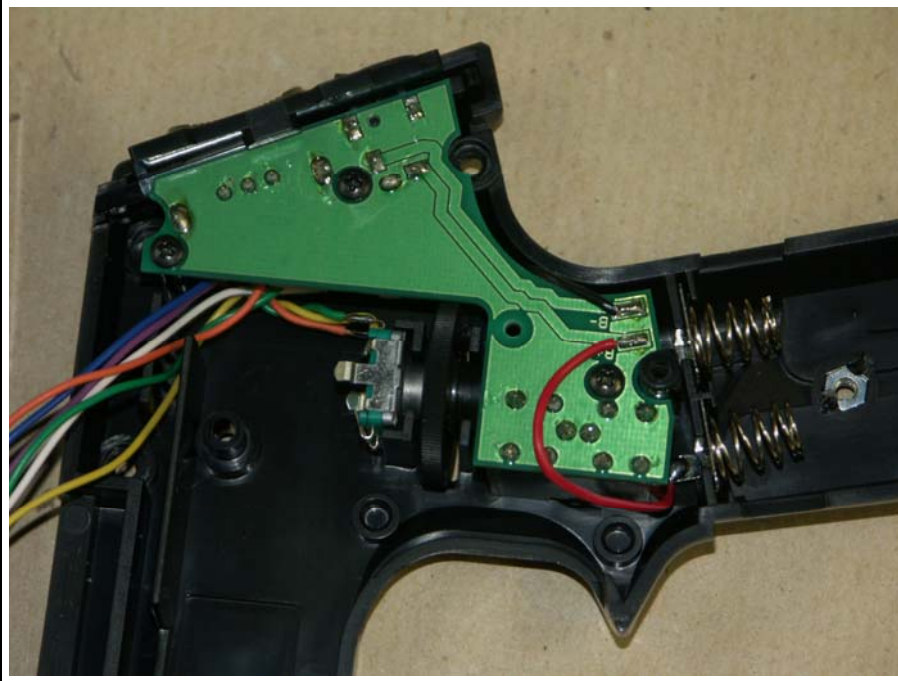
GRIP UNIT
