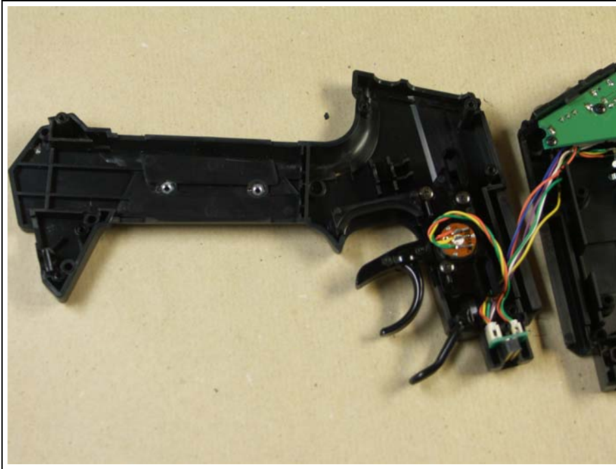
GRIP UNIT
