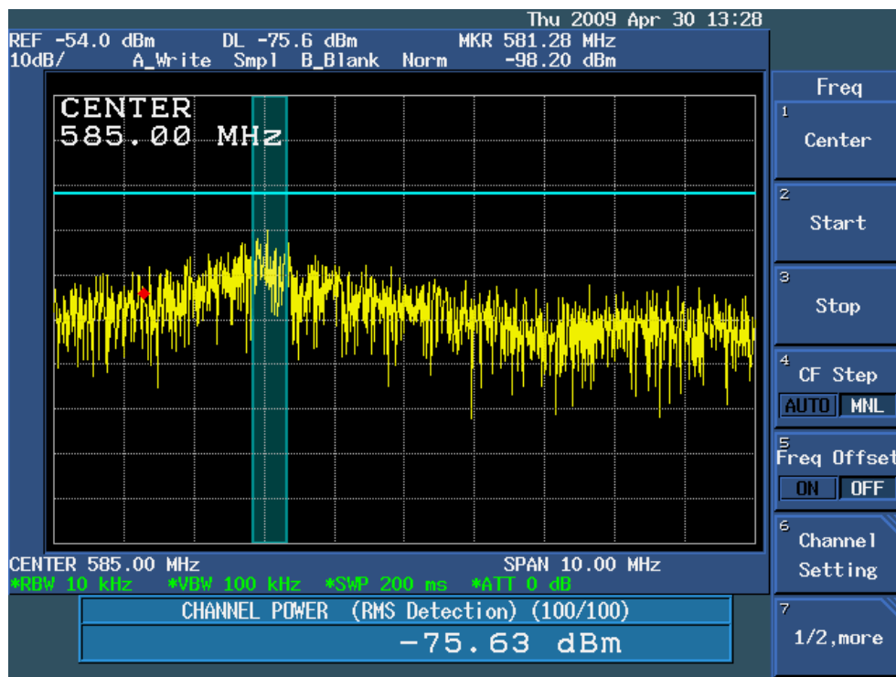
3 rd Harmonic Channel Power (worst 500 KHz segment)
