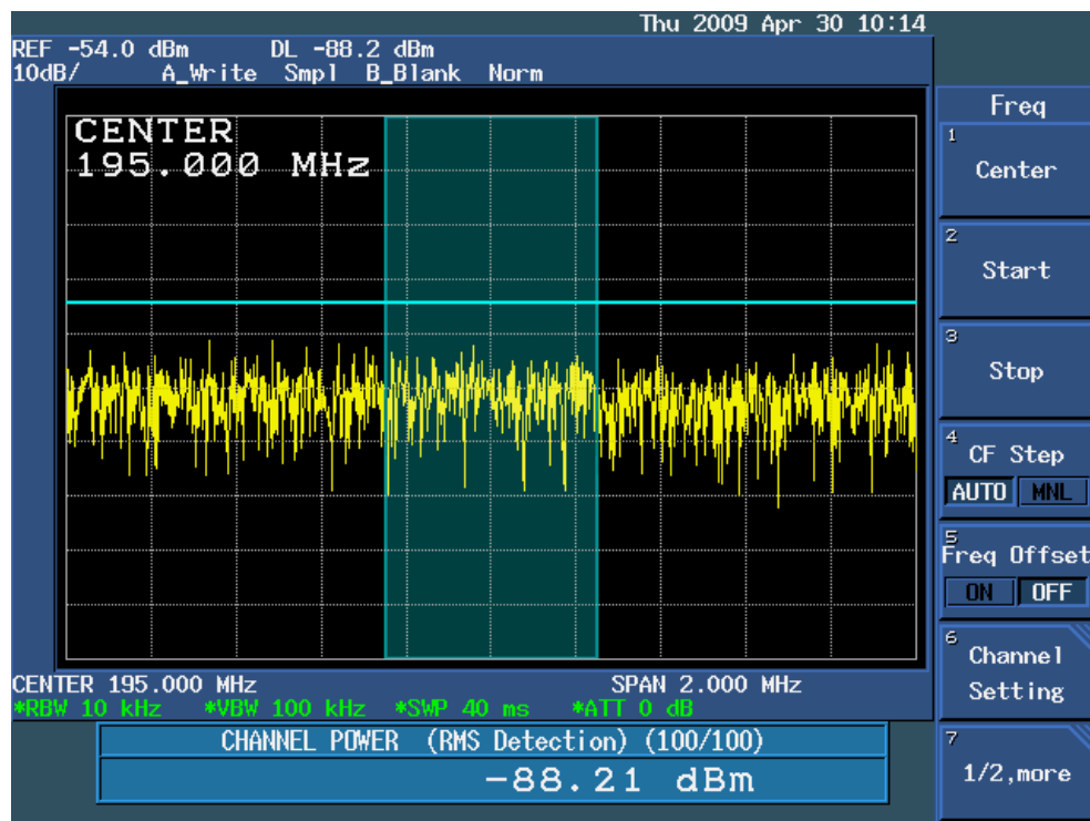
Noise Floor Power (Input Terminated)
