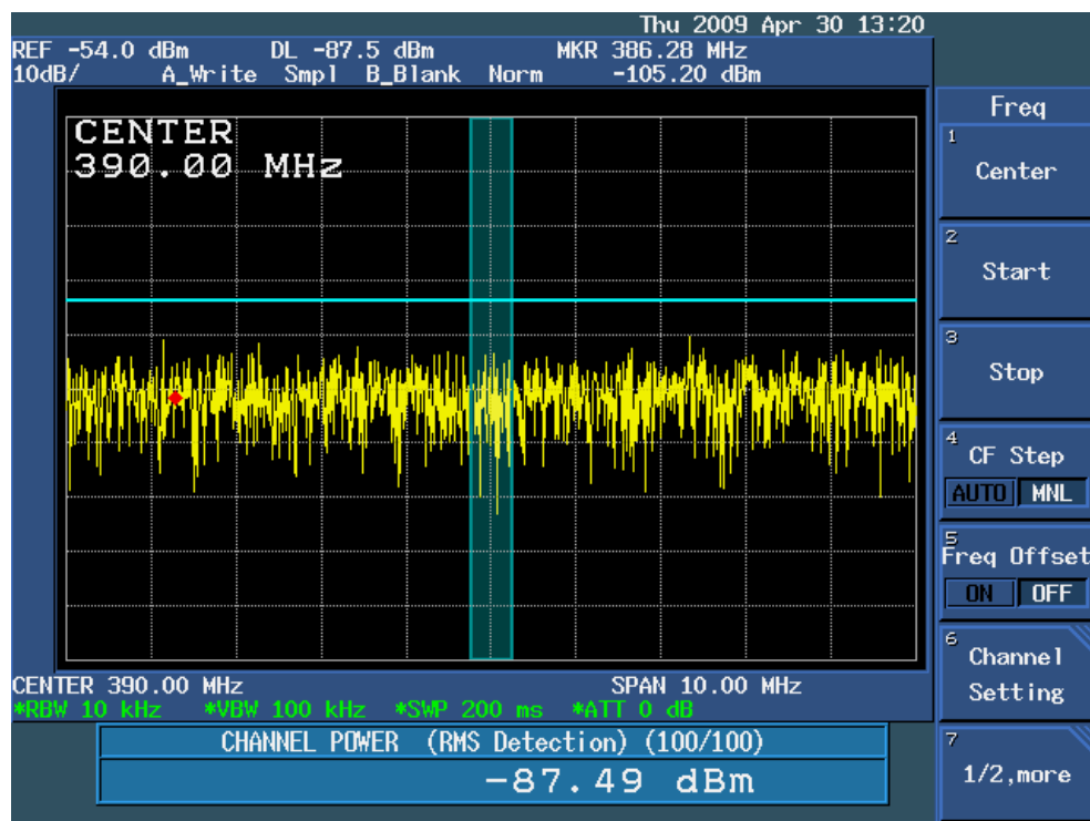
2 nd Harmonic Channel Power (worst 500 KHz segment)
