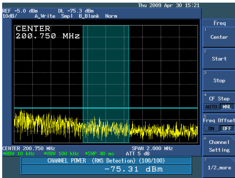
+6 Sub-band Channel power
