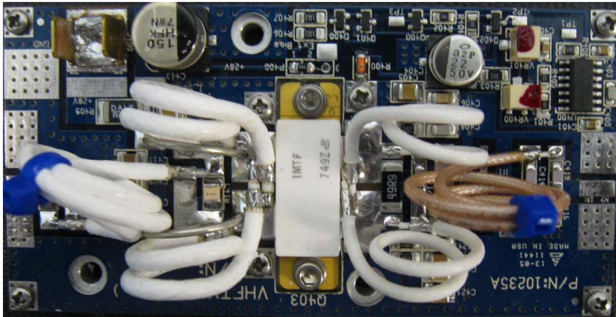
VHF-TV200H Driver (top side):
