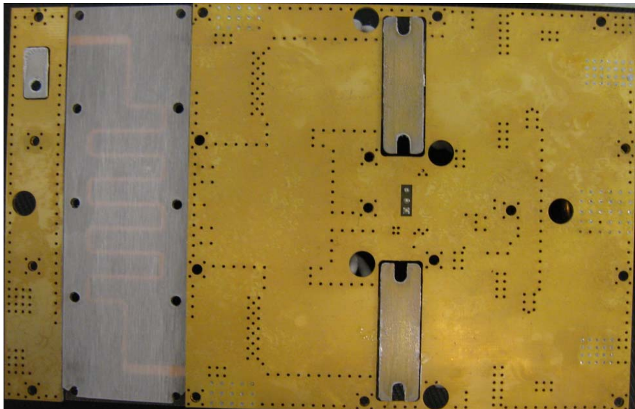
VHF-TV400H Final (bottom side):
