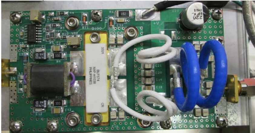
Power Amplifier Construction (lid removed):
