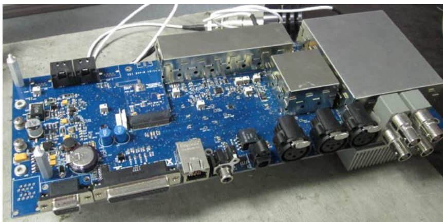
FM Exciter Construction (top):
