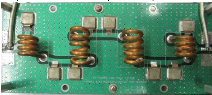
Lowpass Filter Construction (lid removed):
