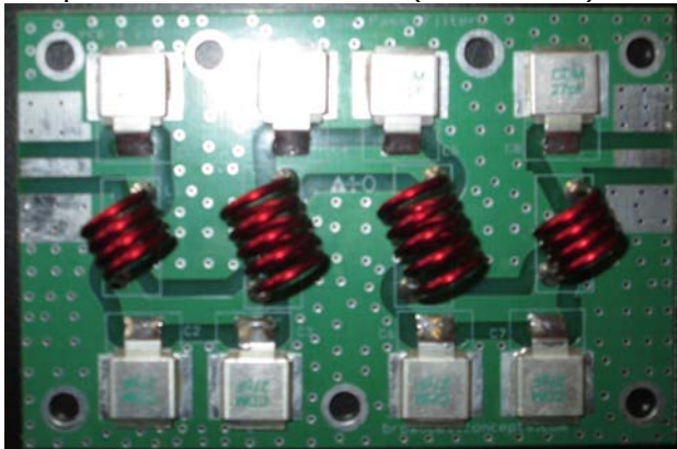
Lowpass Filter Construction (lid removed):
