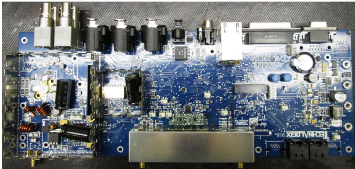
FM Exciter Construction (top):
