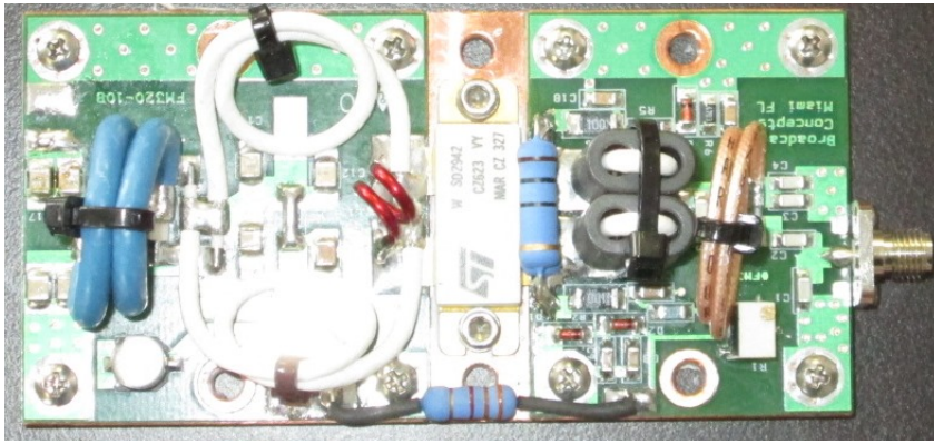
Power Amplifier Construction (lid removed):
