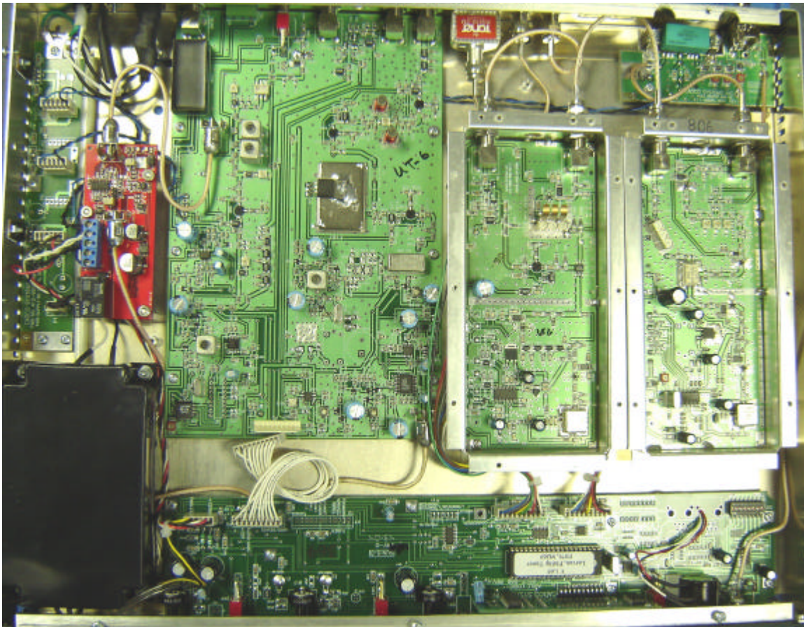
Internal View with Shields of Upconverter and Downconverter Removed:
