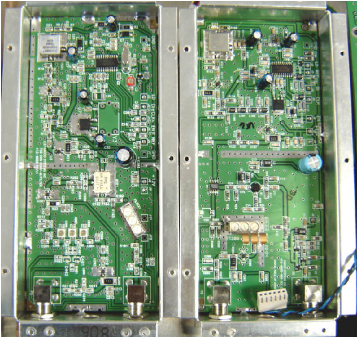
Internal view of Upconverter and Downconverter PCB:
