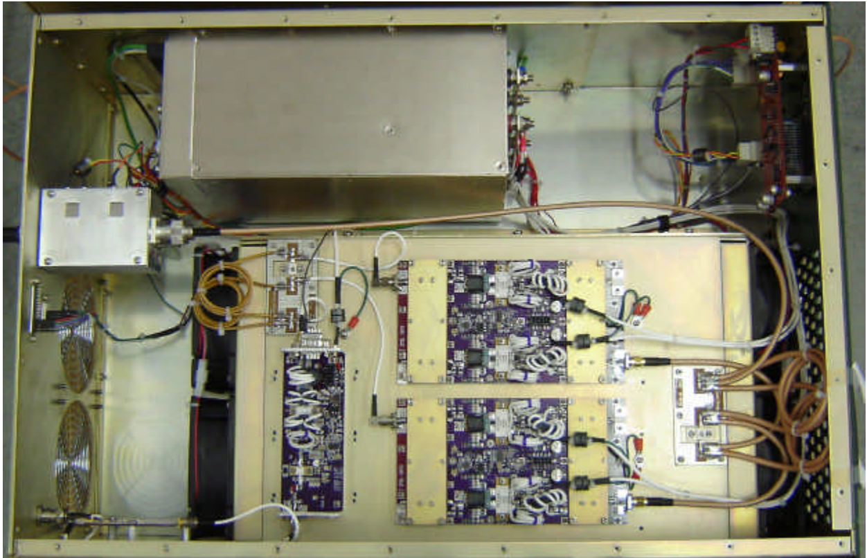
Internal Construction (Shown with optional internal power supply):
