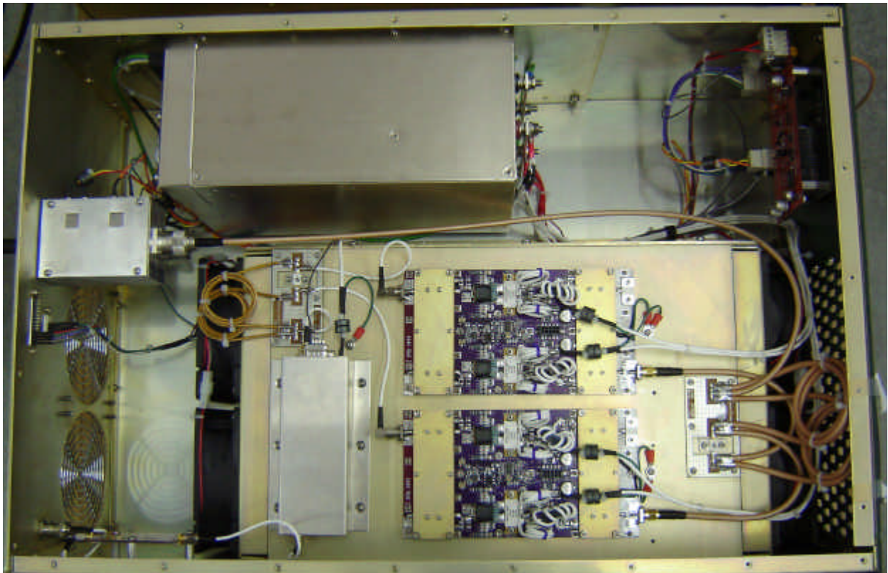
Internal Construction (amplifier pallet lid installed):
