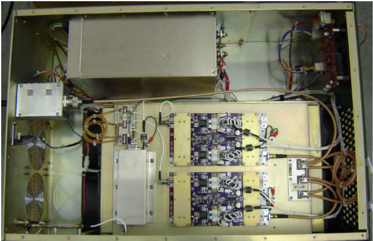
PA Internal Construction (amplifier pallet lid installed):
