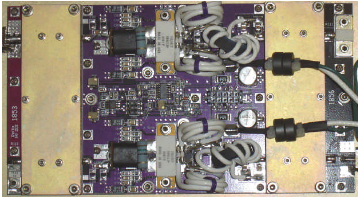
P400-VHF-L (component side with all components):
