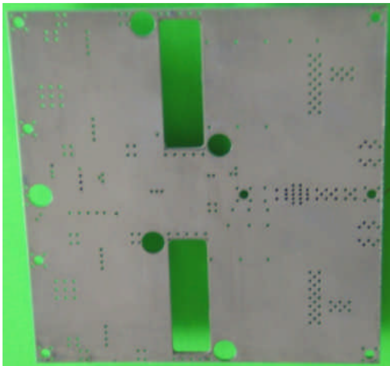
P400-VHF-L (no components get soldered to solder side):
