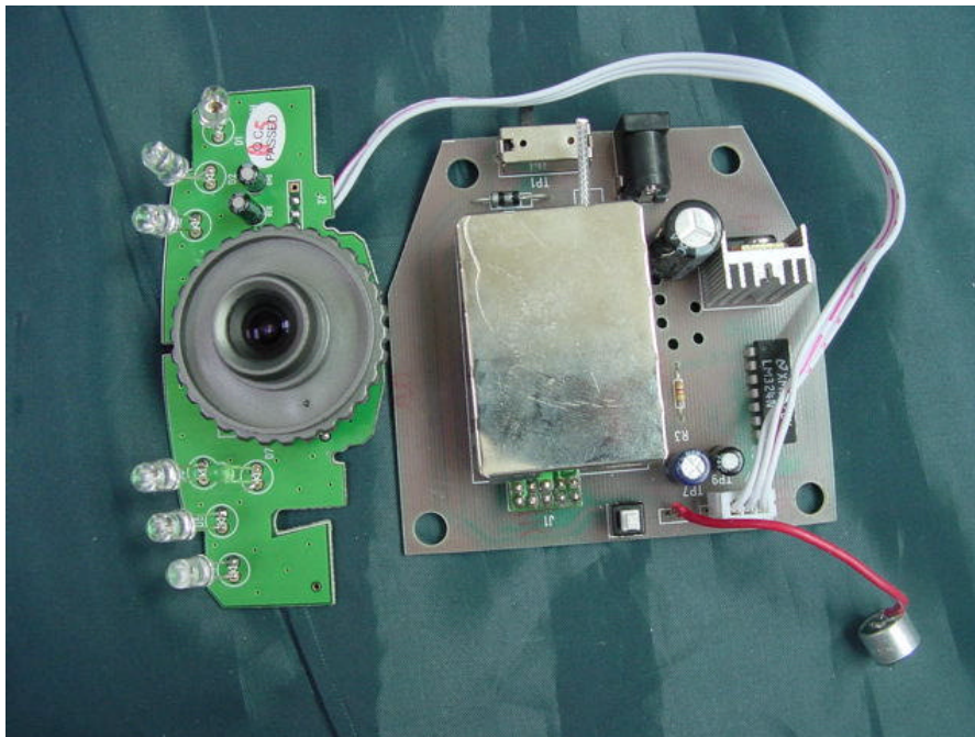
Photo4 PCB of Transmitter
