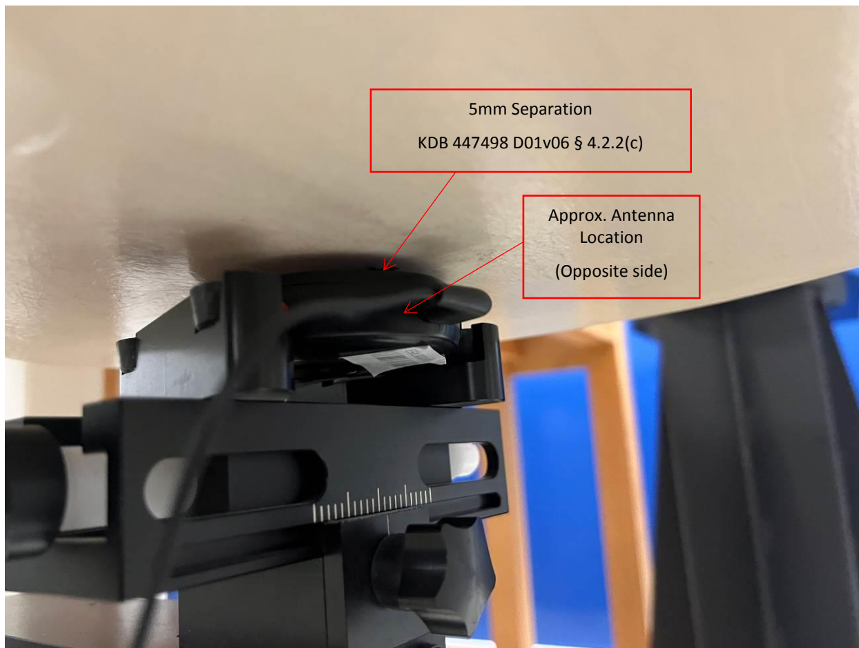
SAR Testing with Headset Accessory
