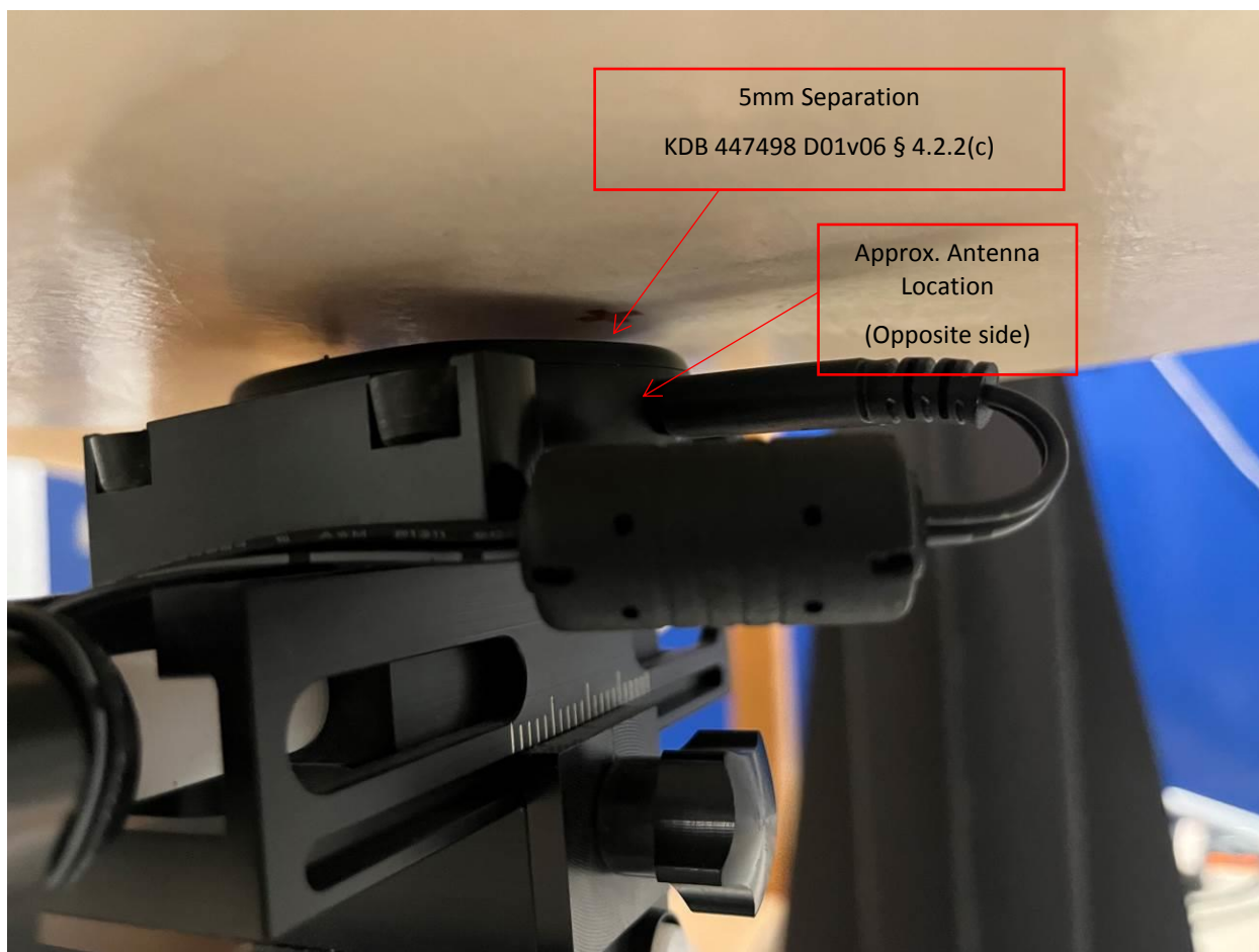
SAR Testing with Charging Accessory
