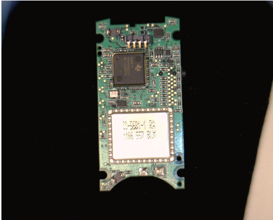
Bottom View of PCBA
