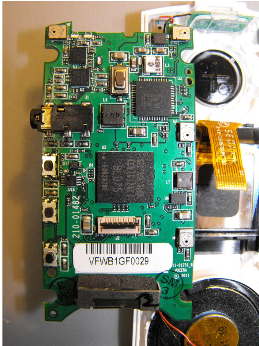
Internal Board Bottom Side
