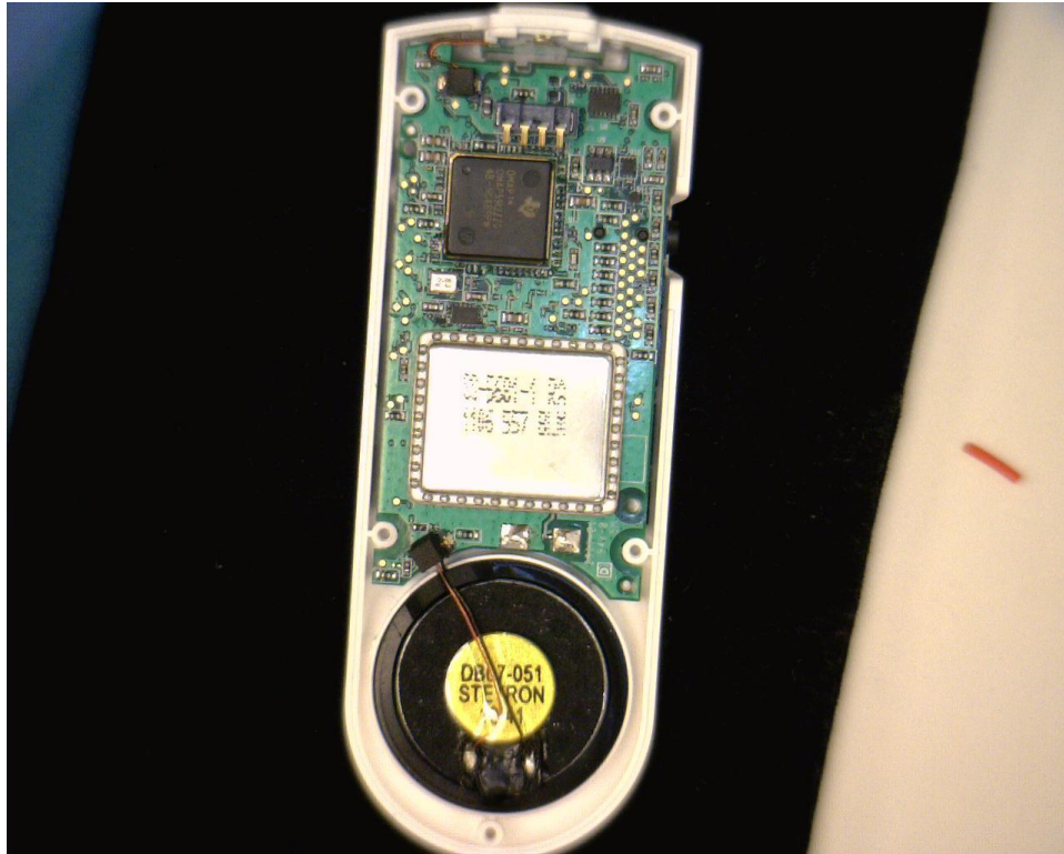
Internal Board Top Side
