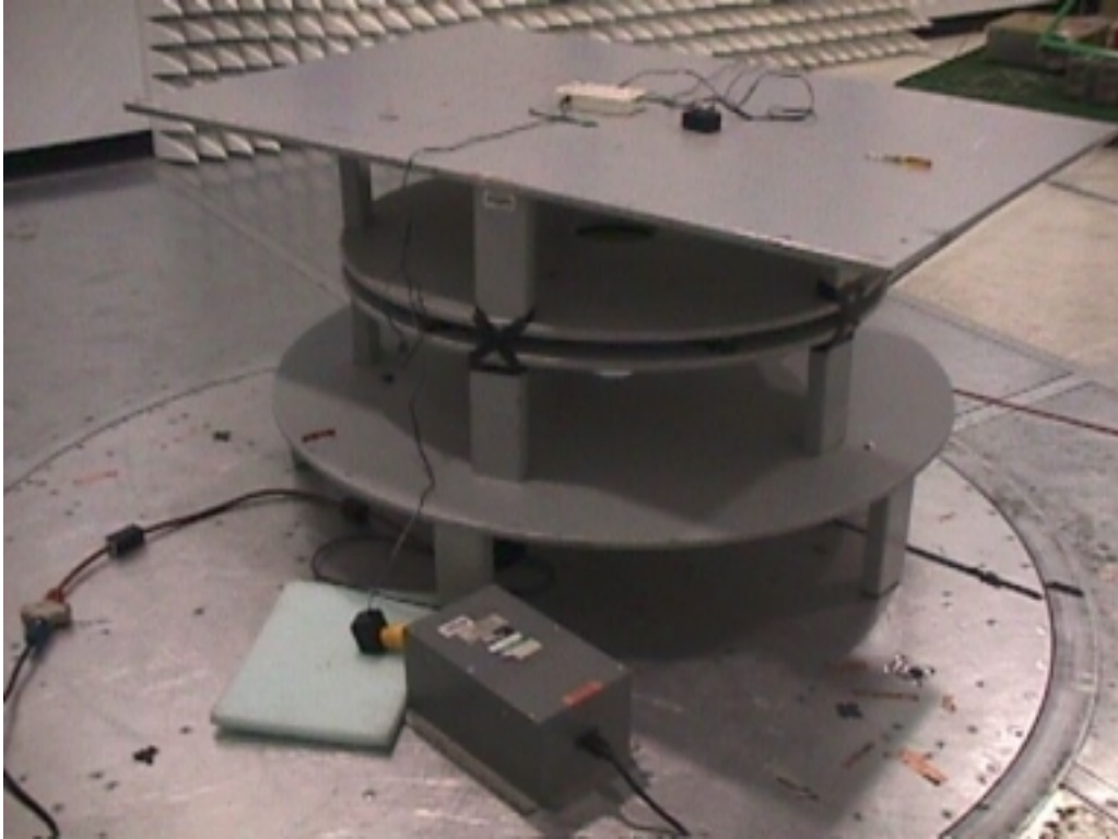
Conducted Emissions Test Configuration
