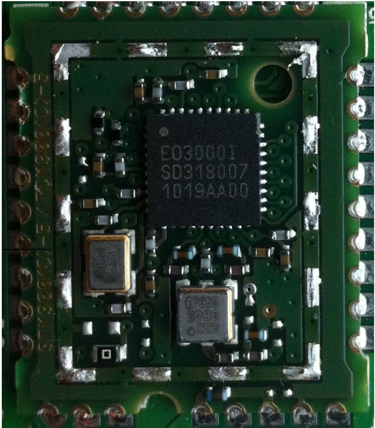
View of the Circuitry Under the RF Shield
