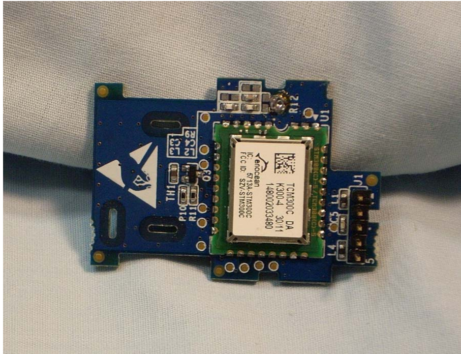
View of the Back Side of the RF PCB
