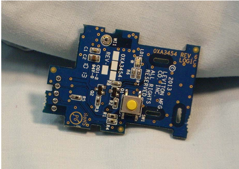
View of the Front Side of the RF PCB
