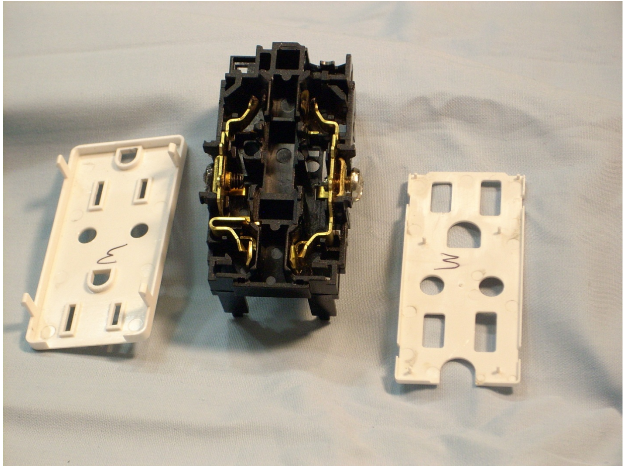
Back View of the Plastic Housing Components of the EUT
