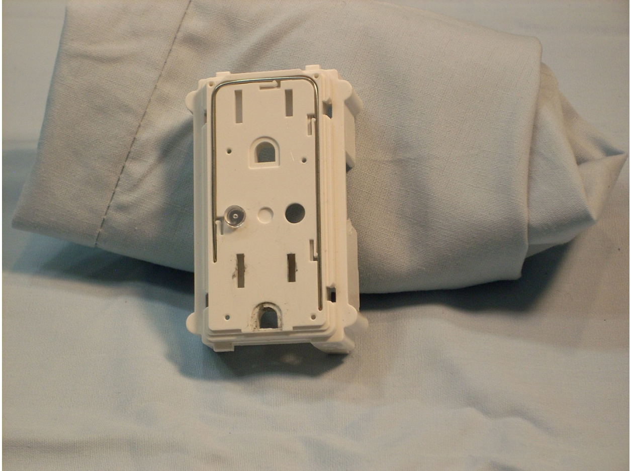
Front View Internal Plastic Housing with Antenna Installed
