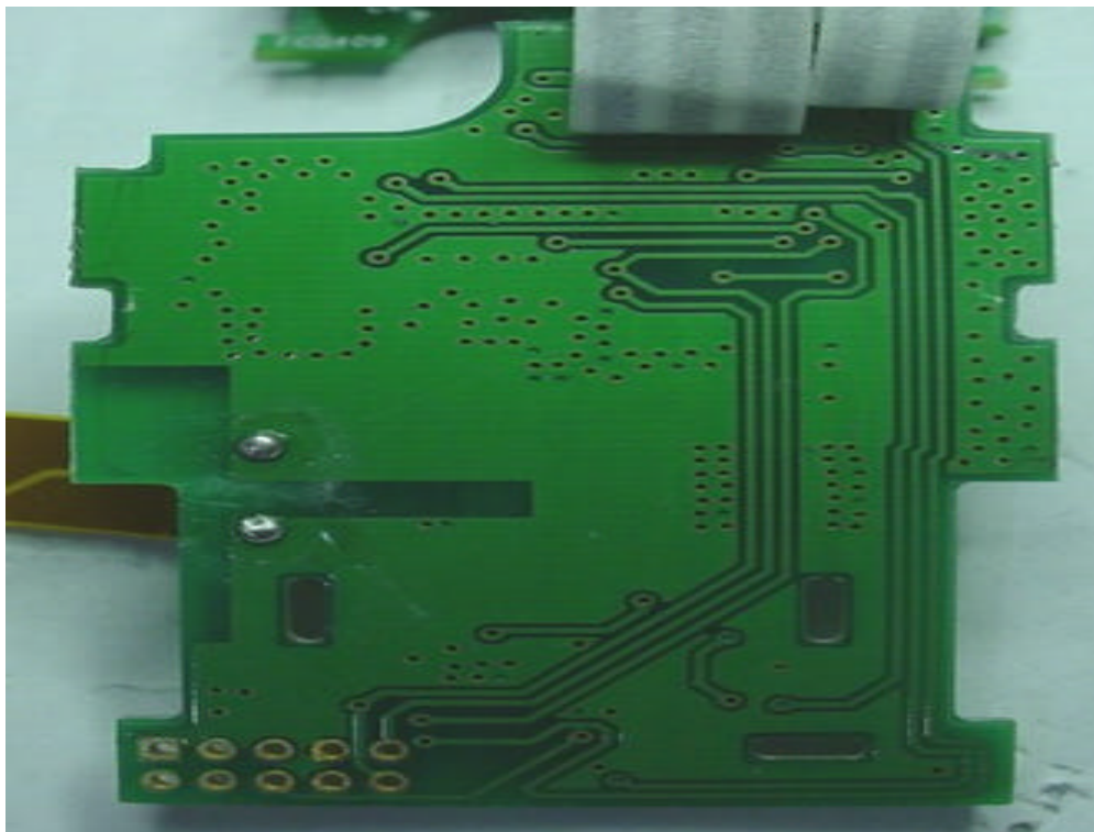
VRR15 Bottom View
