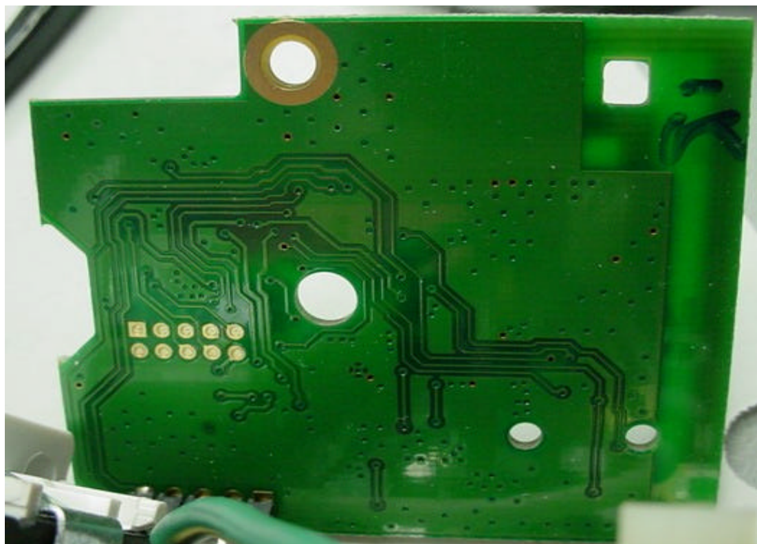
VRP15 Bottom View
