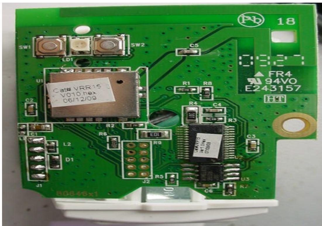
VRP15 Top View
