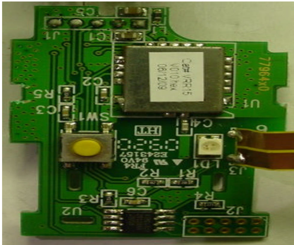
VRR15 Top View
