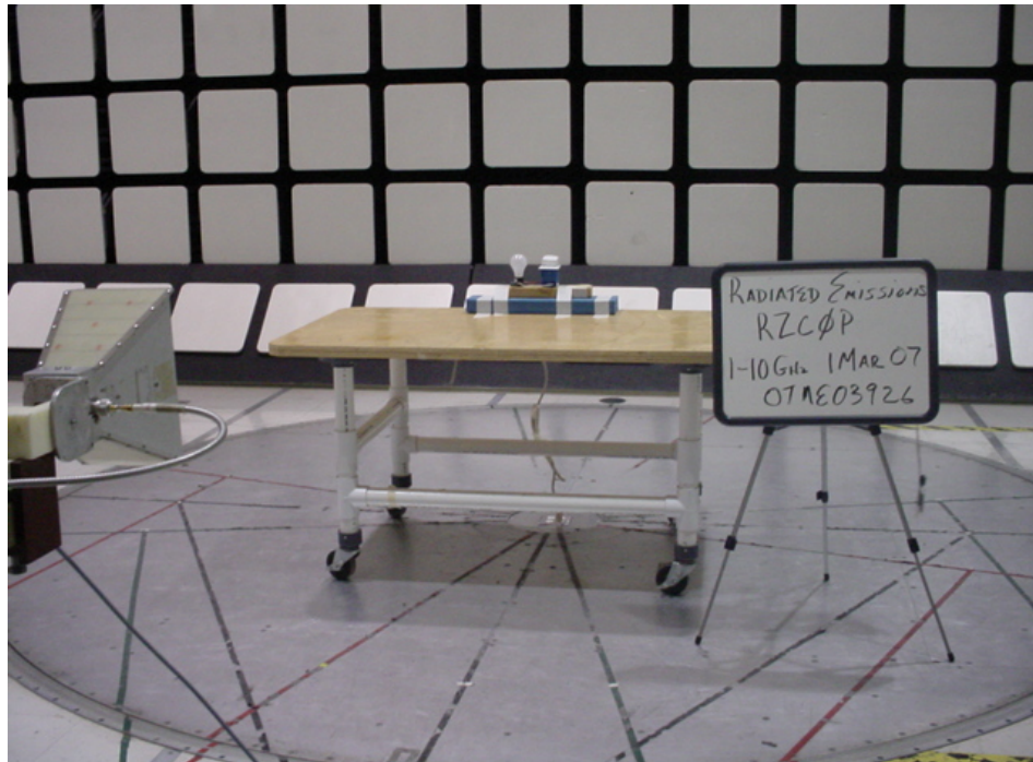
Radiated Emissions 1-10GHz
