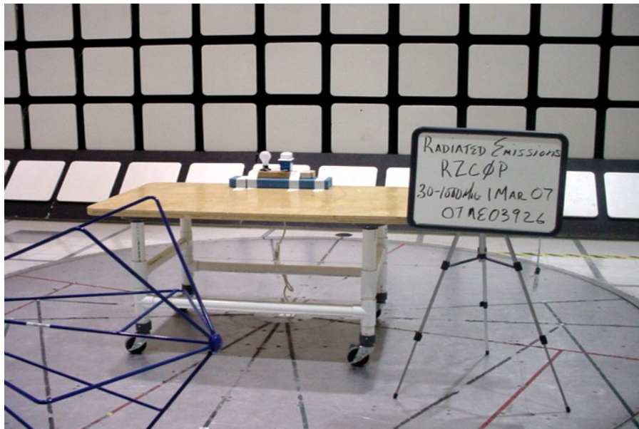
Radiated Emissions 30-1000MHz
