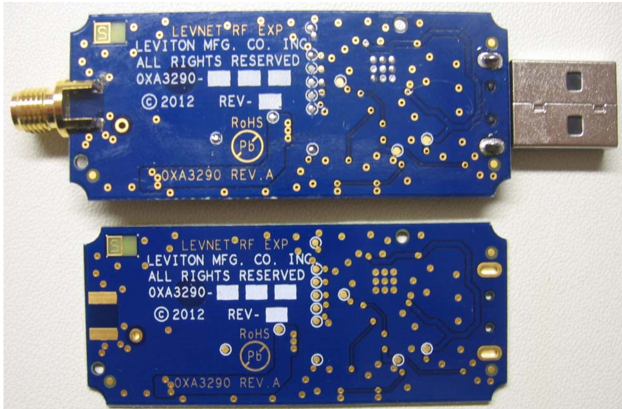
Figure 3. WSCOM-03W Bottom
