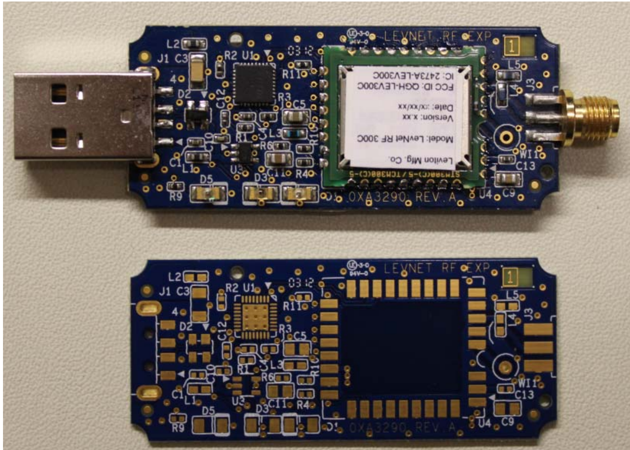
Figure 1. WSCOM-03W Top (Component Side)
