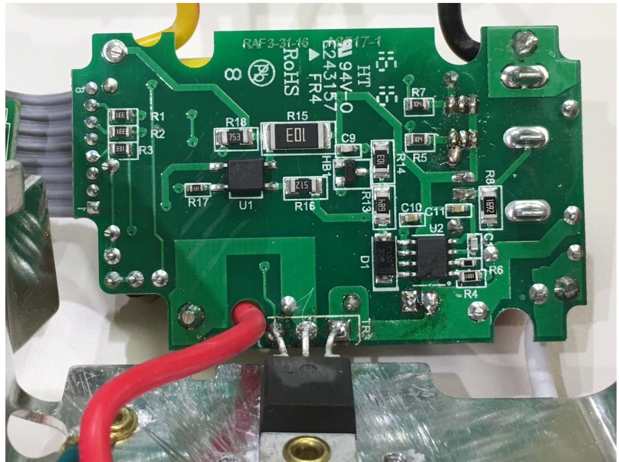
DDF01 AC Mains Board Bottom
