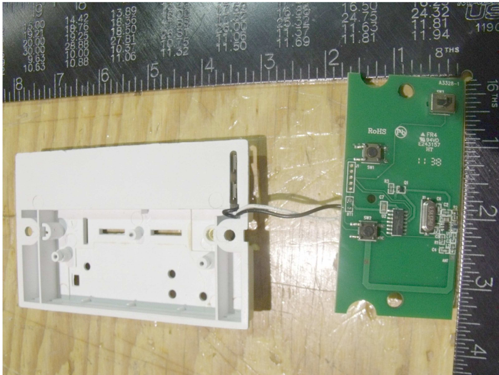
Top view internal photos with enclosure
