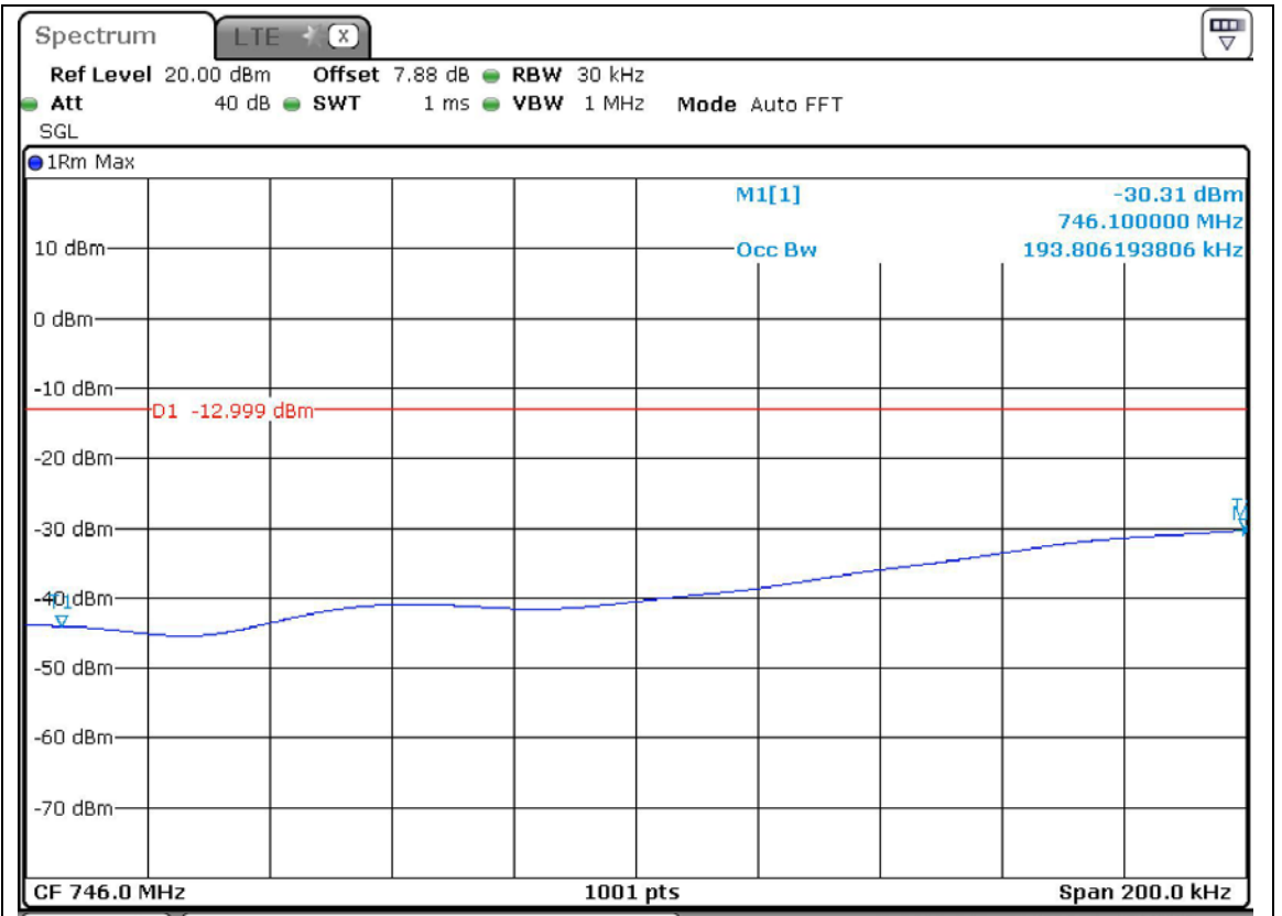
Fig D4 Band 17 TX2 – BW10MHz MIDDLE Channel 64QAM Band Edge Upper
