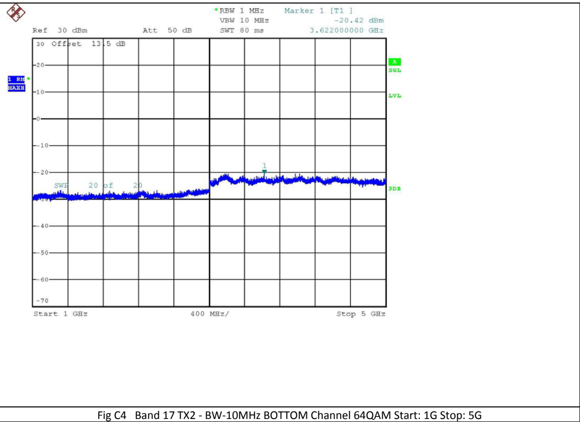
Fig C4 Band 17 TX2 - BW-10MHz BOTTOM Channel 64QAM Start: 1G Stop: 5G
