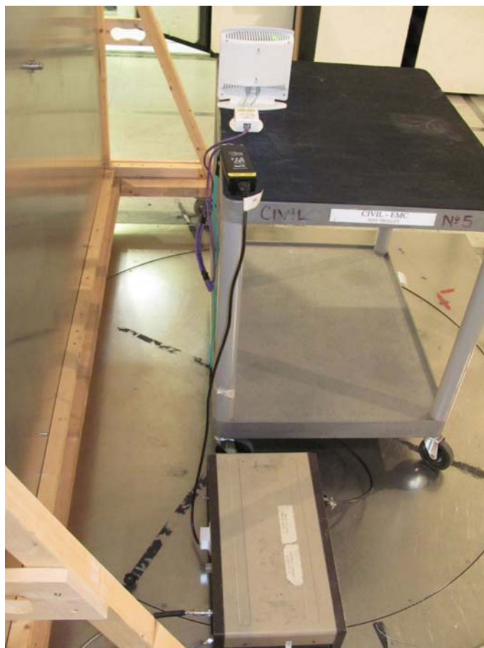
Conducted Emissions
