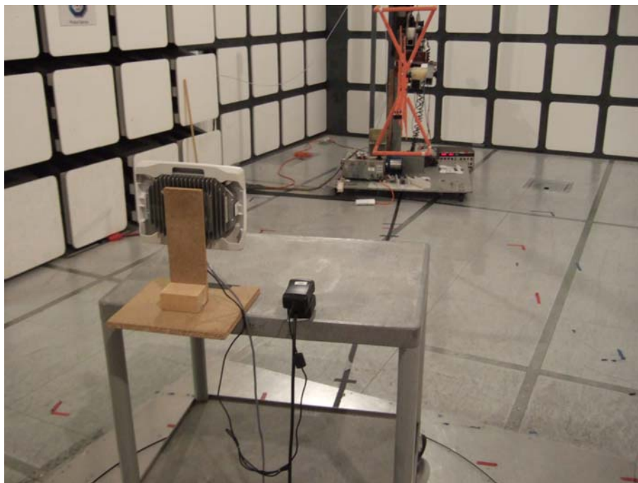
Radiated Emissions - 30MHz to 1GHz (Enclosure Port)
