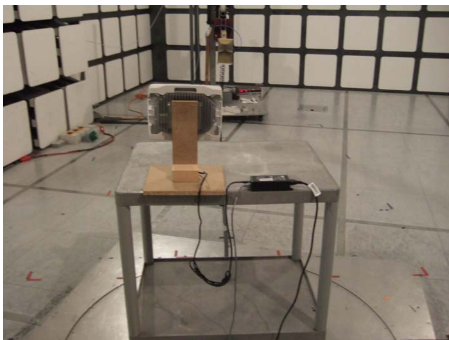
Radiated Emissions – 1GHz to 11GHz (Enclosure Port)
