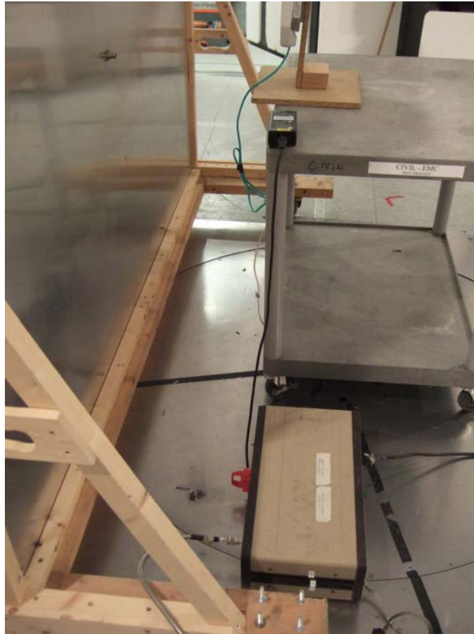
Conducted Emissions – Power Over Ethernet PSU (AC Power Port)
