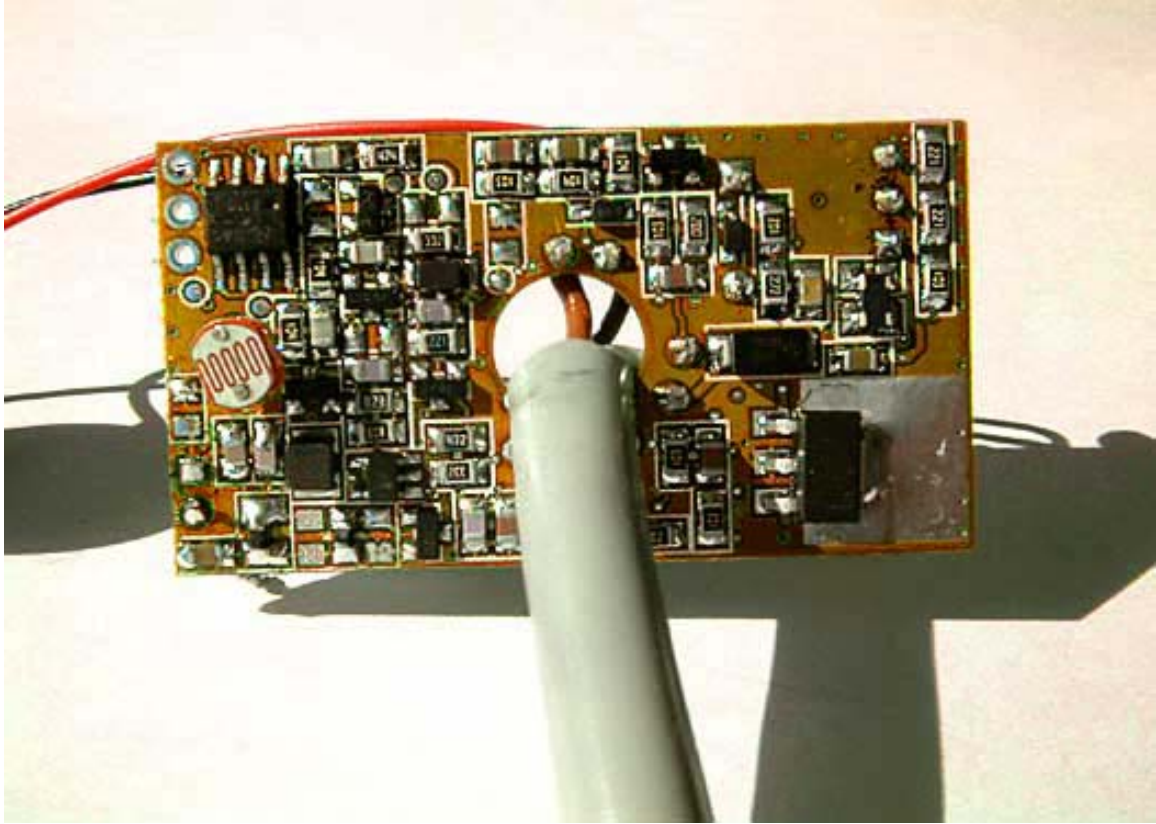
PCB Back 2
