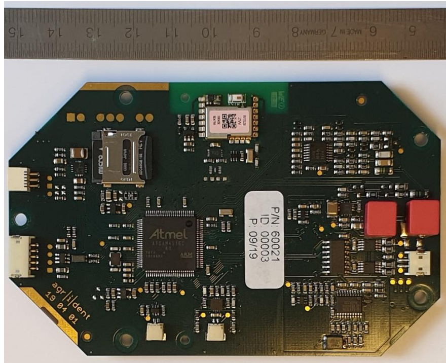
PCB bottom view:
